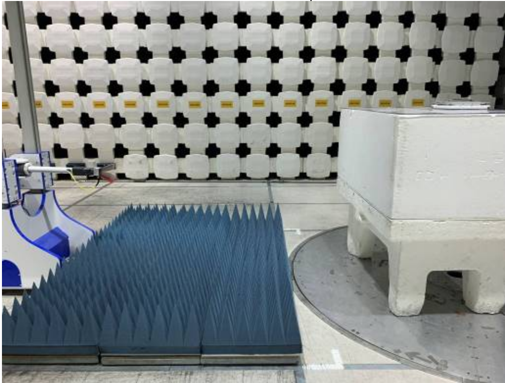
3-18 GHz Test Setup
