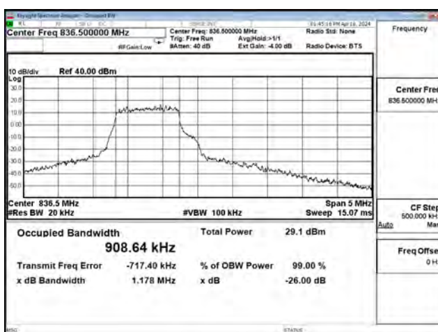
16QAM_CH26915_3M_5RB0
