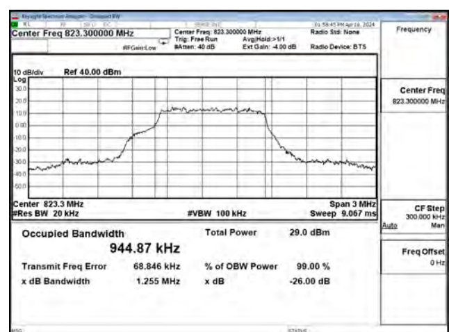
16QAM_CH26783_1.4M_5RB1
