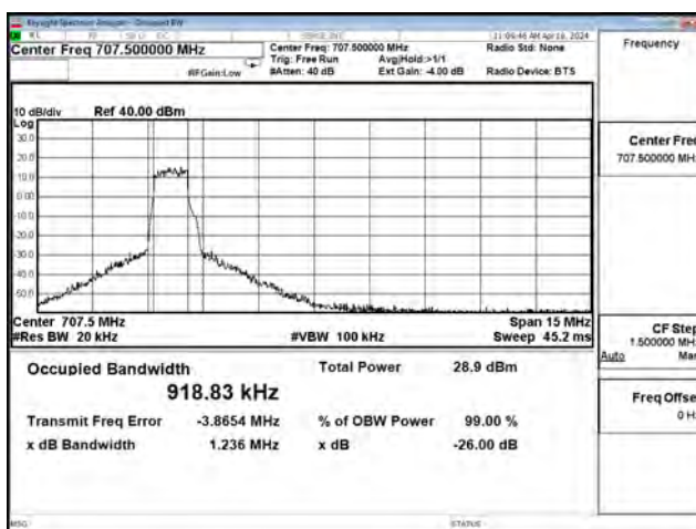
16QAM_CH23095_10M_5RB0
