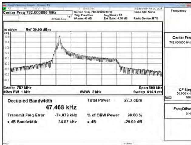
QPSK_CH23230_3.75k_1RB0
