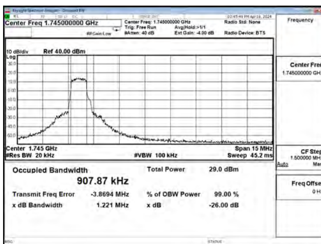
16QAM_CH132322_10M_5RB0
