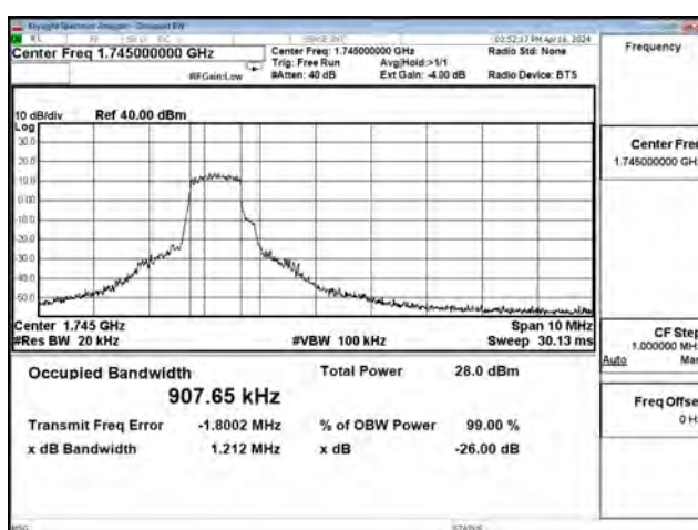
16QAM_CH132322_5M_5RB0
