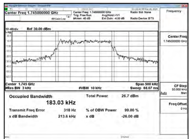
QPSK_CH132322_15k_12RB0
