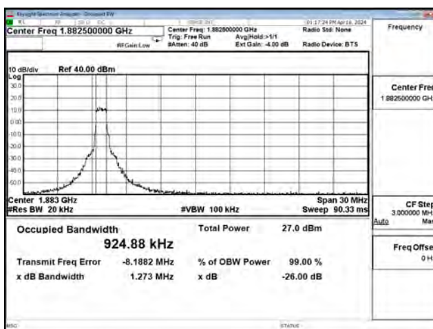
16QAM_CH26365_20M_5RB0
