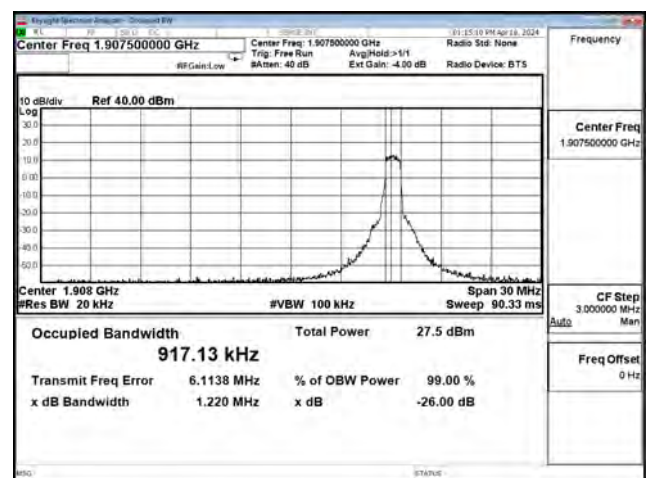
16QAM_CH26615_15M_5RB1
