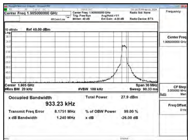
16QAM_CH26590_20M_5RB1
