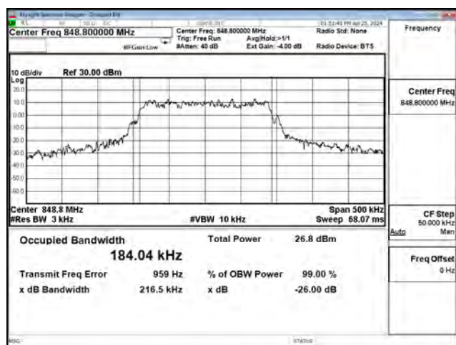
QPSK_CH27038_15k_12RB0
