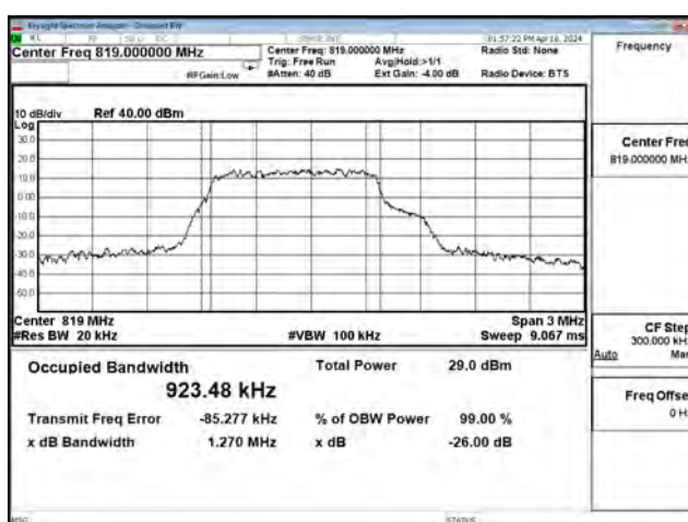
16QAM_CH26740_1.4M_5RB0
