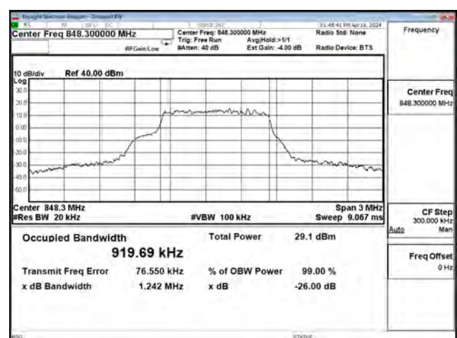
16QAM_CH27033_1.4M_5RB1
