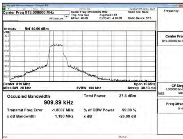
16QAM_CH26740_5M_5RB0
