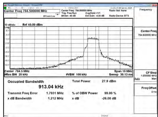
16QAM_CH23255_5M_5RB1
