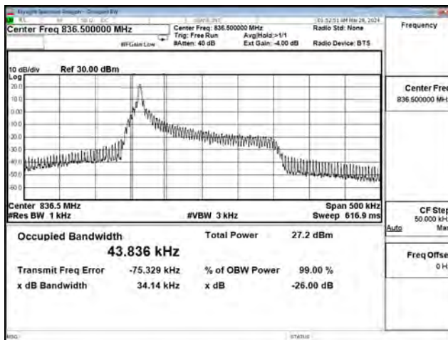
QPSK_CH26915_3.75k_1RB0
