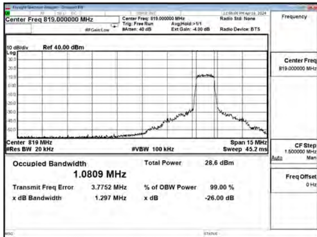
QPSK_CH26740_10M_5RB0_high
