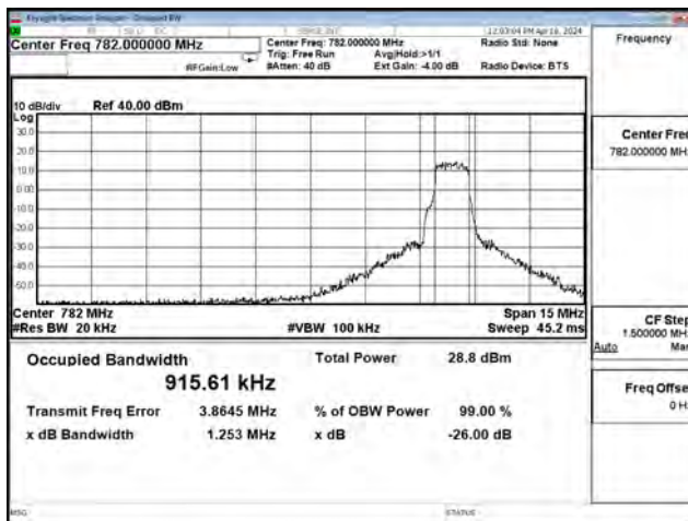
16QAM_CH23230_10M_5RB0_high
