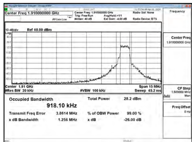
16QAM_CH26640_10M_5RB1
