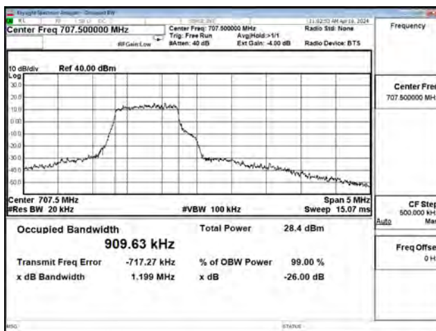
16QAM_CH23095_3M_5RB0
