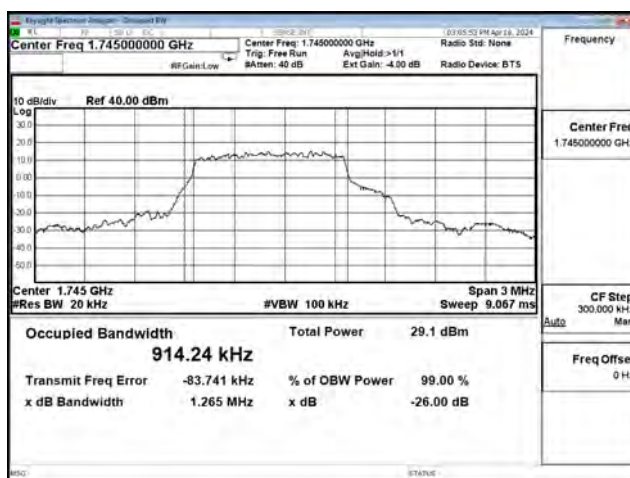
16QAM_CH132322_1.4M_5RB0
