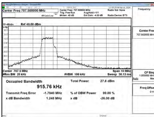
16QAM_CH23095_5M_5RB0
