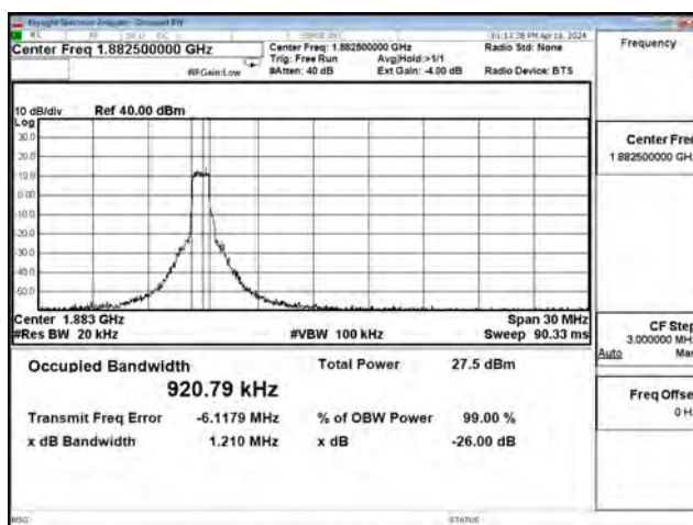
16QAM_CH26365_15M_5RB0
