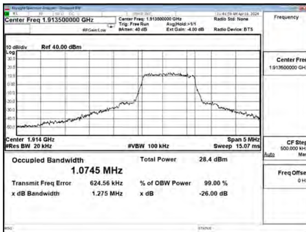
16QAM_CH26365_3M_5RB0
