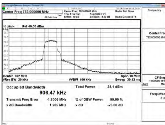
16QAM_CH23230_5M_5RB0
