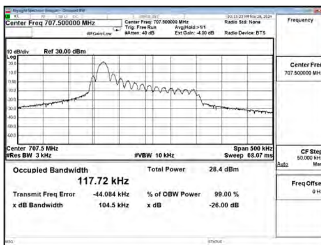
QPSK_CH23095_15k_1RB0
