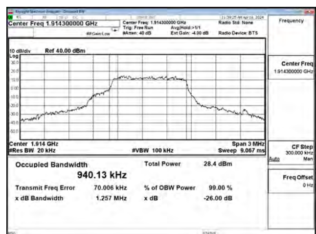
16QAM_CH26683_1.4M_5RB1
