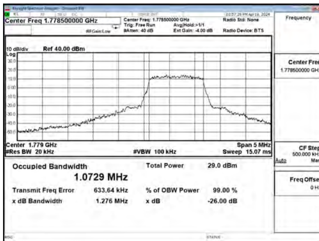
16QAM_CH132322_3M_5RB0
