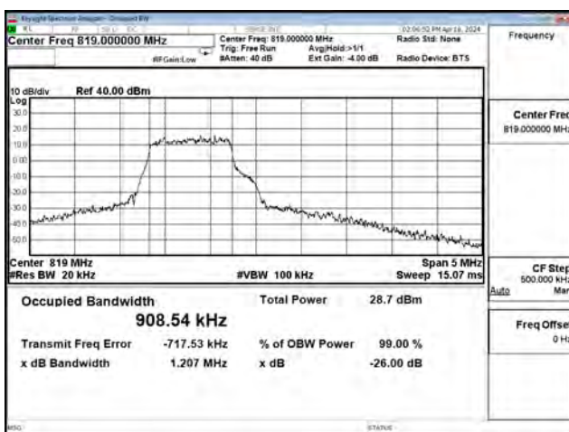
16QAM_CH26740_3M_5RB0
