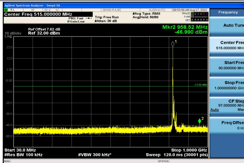
Band5-10MHz-QPSK-20450-1RB#0-30~1000MHz
