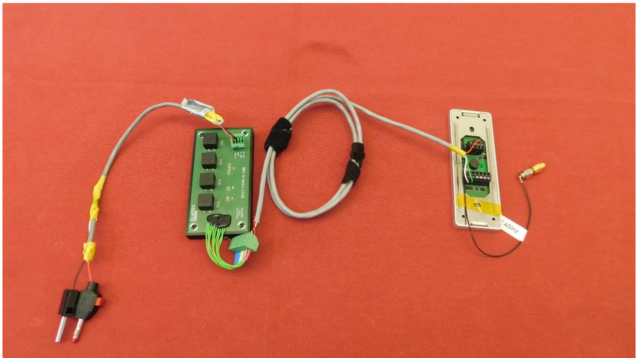
Picture 15: EUT connected with Wiegand adapter rear view
