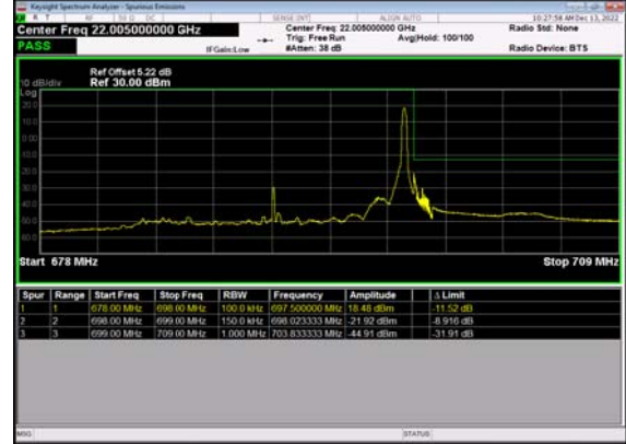
N71(15M)_DFT-s- OFDM QPSK Edge 1RB Right High CH
