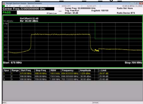
N71(15M)_DFT-s- OFDM BPSK Outer Full High CH
