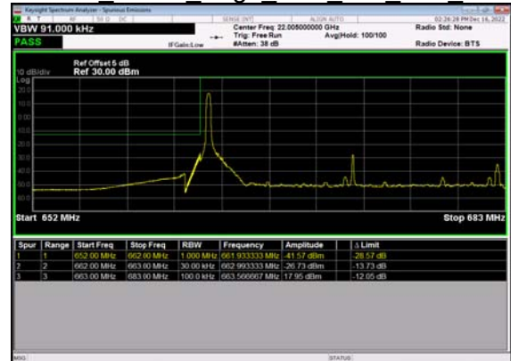
N71(20M)_DFT-s- OFDM QPSK Edge 1RB Left Low CH
