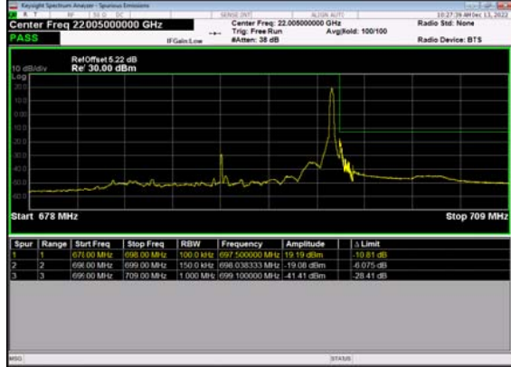
N71(15M)_DFT-s- OFDM BPSK Edge 1RB Right High CH
