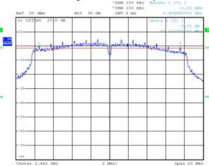
Figure 6-6: 6 dB Bandwidth
