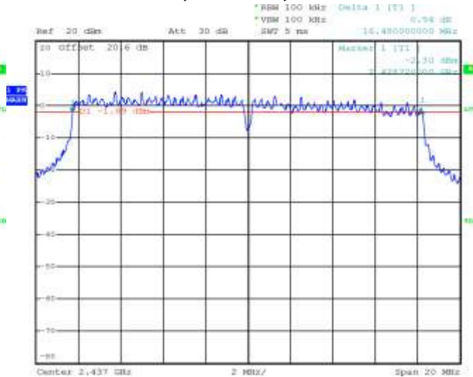
Figure 6-8: 6 dB Bandwidth
