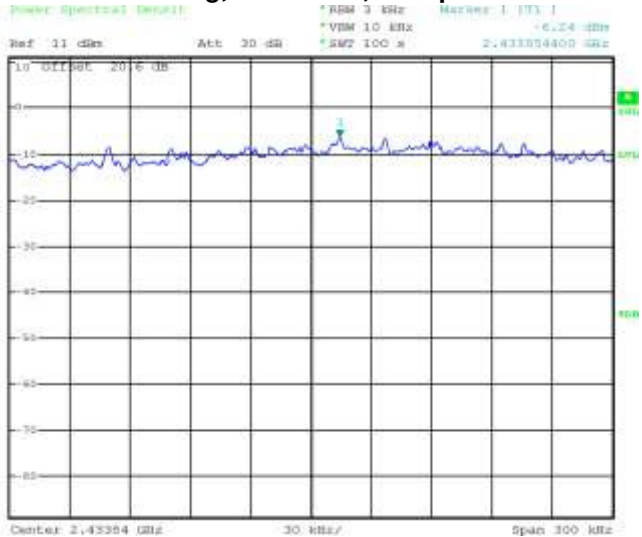
Figure 6-20: Peak Power Spectral Density 802.11g, Channel 6, 6 Mbps
