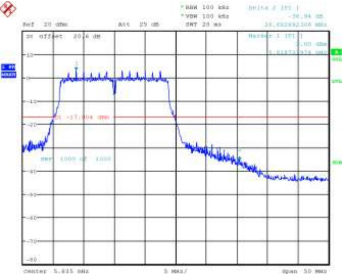
Figure 7-21: Band Edge Compliance 802.11n, Channel 165, 6 Mbps
