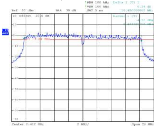
Figure 6-7: 6 dB Bandwidth
