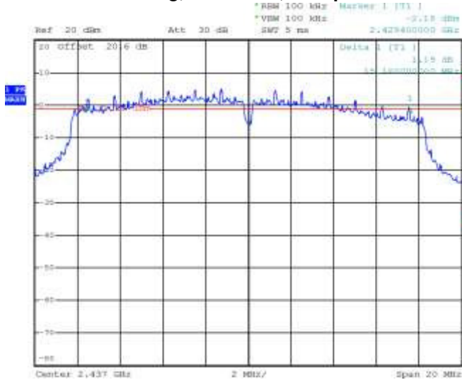
Figure 6-5: 6 dB Bandwidth
