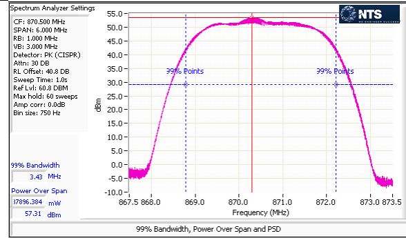
Port 1 – LTE – 16QAM – 3M – Low Channel – Peak
