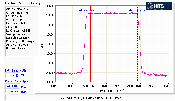
Port 1 – LTE – 16QAM – 5M – High Channel – Average
