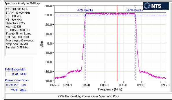
Port 1 – LTE – 16QAM – 15M – Center Channel – Average
