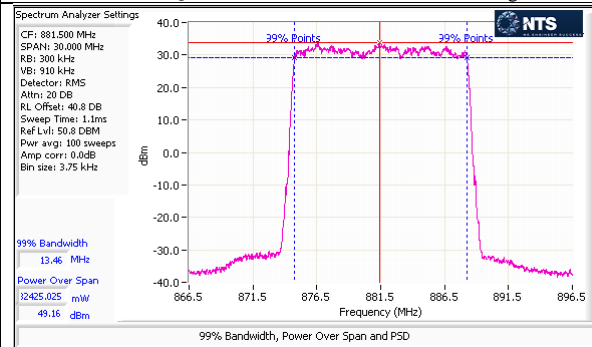
Port 3 – LTE – 64QAM – 15M – Center Channel – Average
