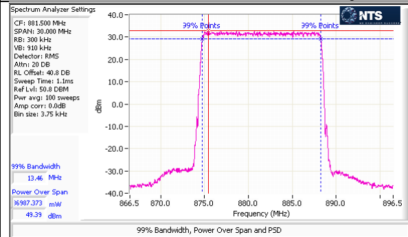
Port 1 – LTE – 64QAM – 15M – Center Channel – Average
