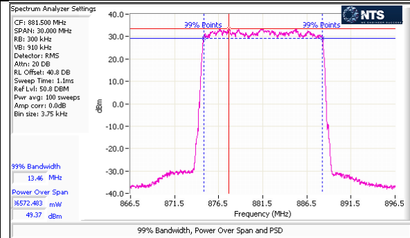
Port 5 – LTE – 64QAM – 15M – Center Channel – Average
