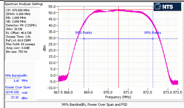
Port 1 – LTE – 64QAM – 3M – Low Channel – Peak
