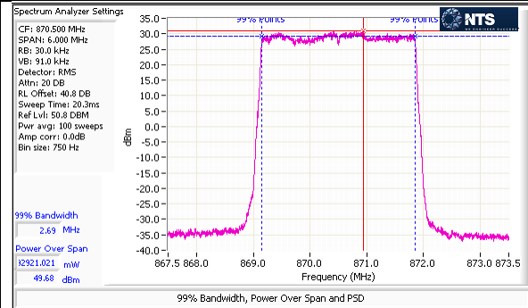
Port 1 – LTE – 64QAM – 3M – Low Channel – Average
