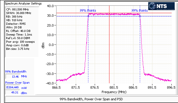
Port 5 – LTE – 16QAM – 15M – Center Channel – Average
