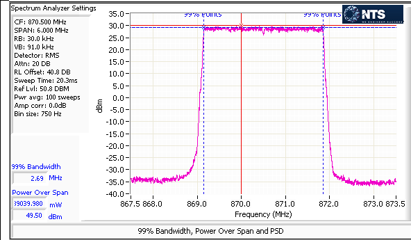
Port 1 – LTE – 16QAM – 3M – Low Channel – Average
