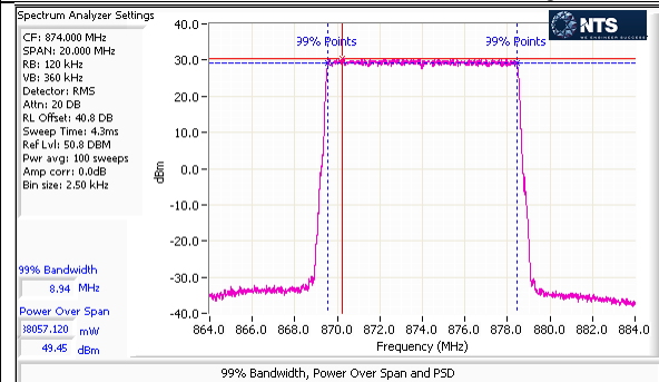
Port 1 – LTE – 64QAM – 10M – Low Channel – Average
