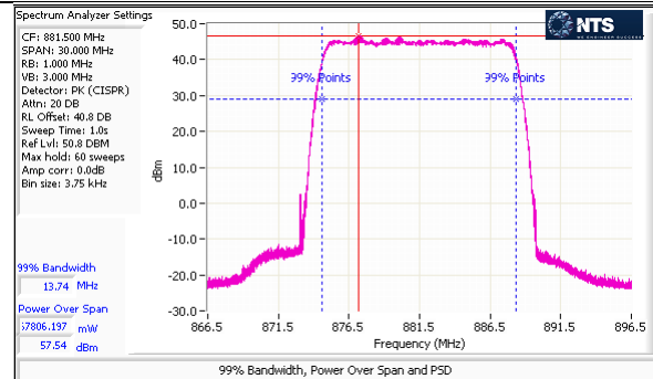
Port 5 – LTE – 64QAM – 15M – Center Channel – Peak
