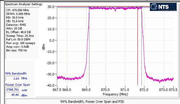
Port 1 – LTE – 64QAM – 3M – Low Channel – Average
