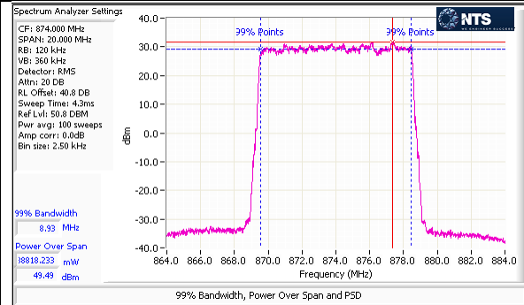
Port 1 – LTE – 64QAM – 10M – Low Channel – Average
