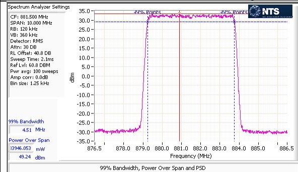
Port 3 – LTE – 64QAM – 5M – Center Channel – Average
