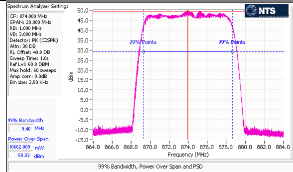
Port 1 – LTE – 64QAM – 10M – Low Channel – Peak
