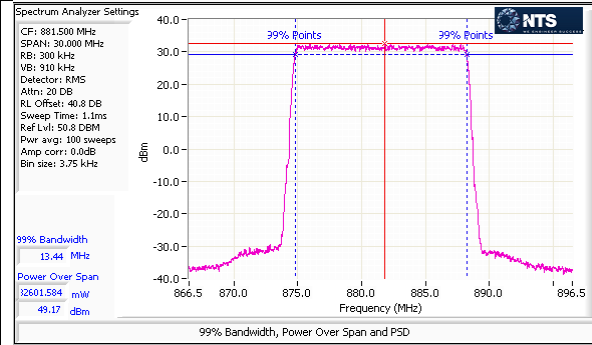
Port 3 – LTE – 16QAM – 15M – Center Channel – Average
