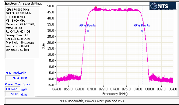
Port 1 – LTE – 16QAM – 10M – Low Channel – Peak
