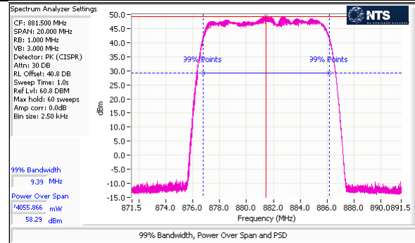
Port 5 – LTE – 64QAM – 10M – Center Channel – Peak
