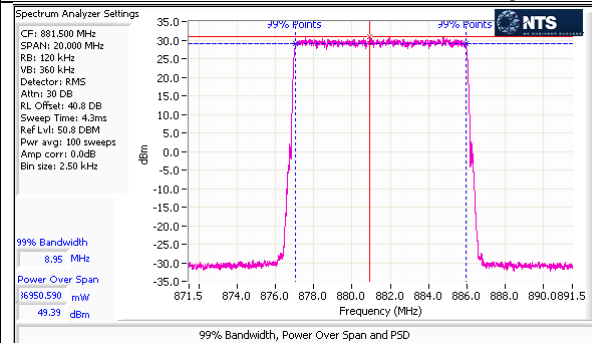
Port 5 – LTE – 64QAM – 10M – Center Channel – Average
