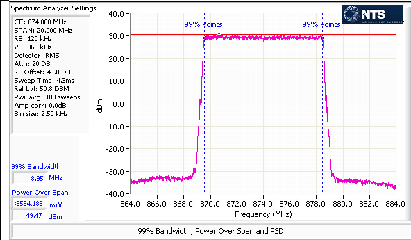
Port 1 – LTE – 16QAM – 10M – Low Channel – Average
