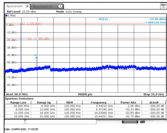
Figure 7.5.1.2-2: MCH – 30MHz–25GHz
