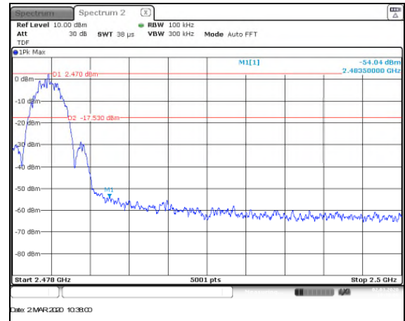
Figure 7.5.1.2-5: Upper Band-edge
