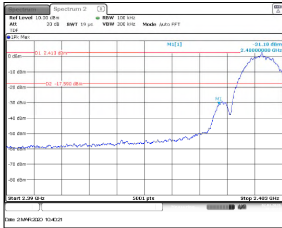
Figure 7.5.1.2-4: Lower Band-edge
