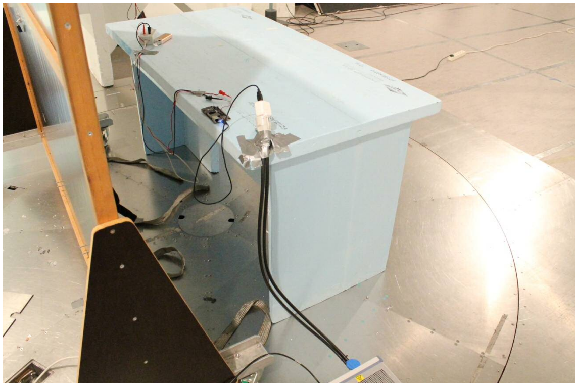
Photograph 6. Conducted Emissions
