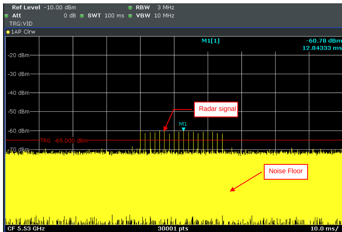
Radar Signal 0
