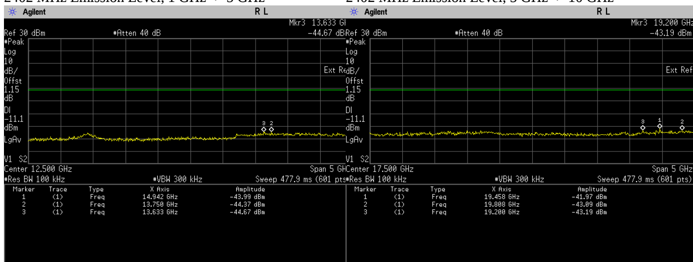
Conducted Emissions(Peak). Bluetooth LE, Frequency 2402 MHz Emission Level, 10 GHz -> 15 GHz
