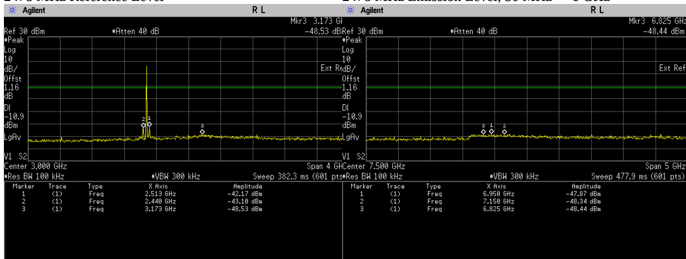
Conducted Emissions(Peak). Bluetooth LE, Frequency 2478 MHz Emission Level, 1 GHz -> 5 GHz
