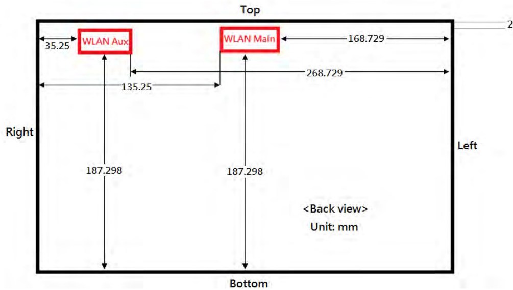
Fig.7 Antenna position of EUT (Back view)
