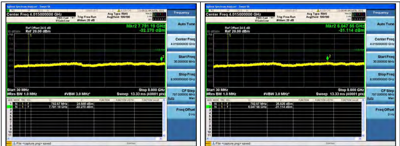
Band13 / 5MHz / High CH / 64QAM
