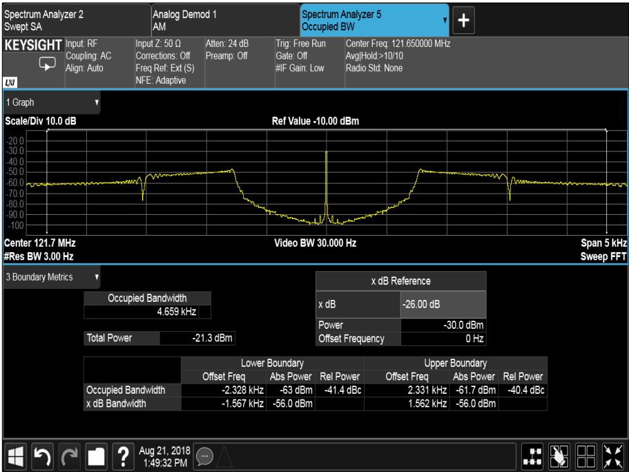
Figure 14 - 99% Occupied Bandwidth
