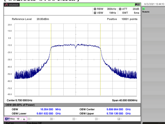
[ 802.11a/ 5700 MHz ]
