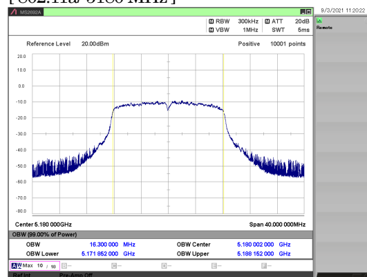
[ 802.11a/ 5180 MHz ]
