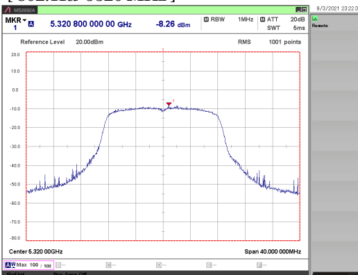
[ 802.11a/ 5320 MHz ]
