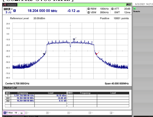
[ 802.11a/ 5700 MHz ]
