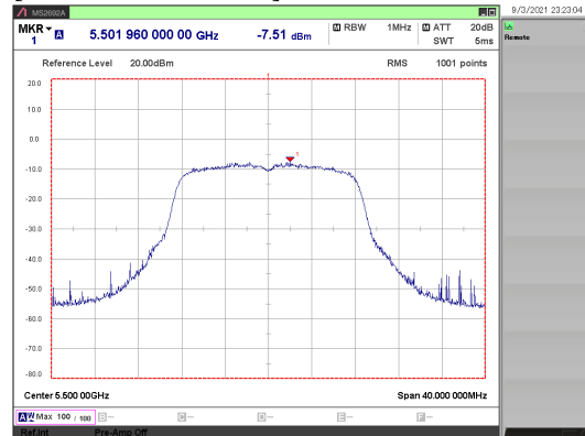
[ 802.11a/ 5500 MHz ]
