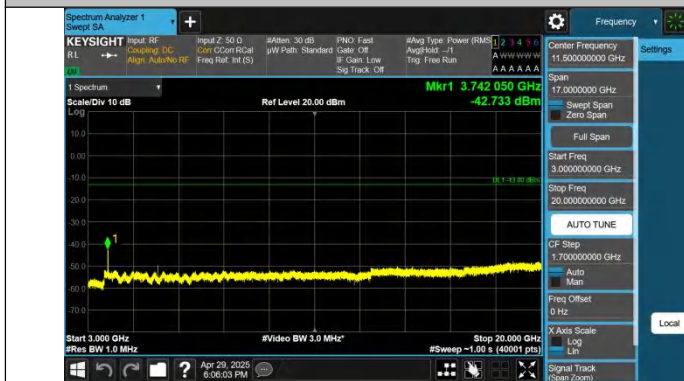
Band2-20MHz-QPSK-18900-1RB#0-3000~20000-PASS
