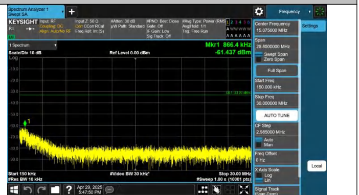
Band2-10MHz-QPSK-18650-1RB#0-0.15~30-PASS
