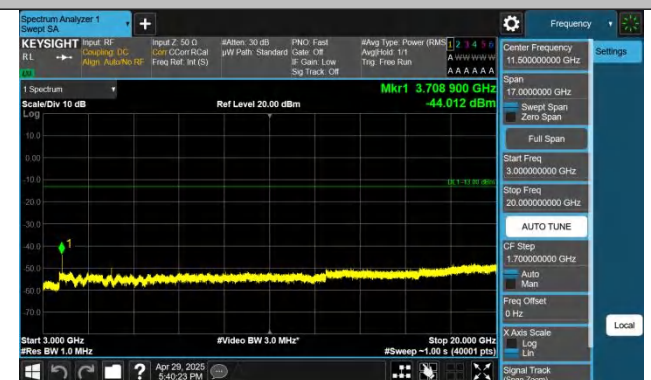
Band2-5MHz-QPSK-18625-1RB#24-3000~20000-PASS
