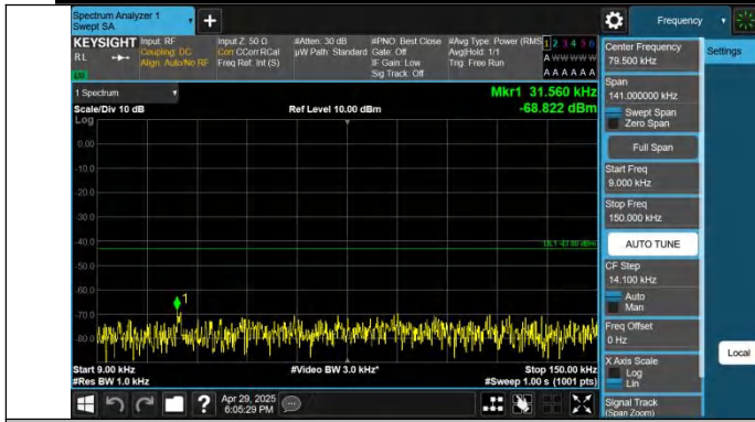
Band2-20MHz-QPSK-18900-1RB#0-0.009~0.15-PASS
