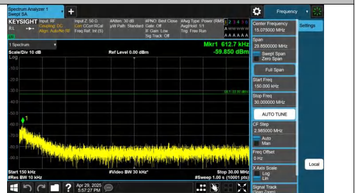
Band2-15MHz-QPSK-18900-1RB#0-0.15~30-PASS
