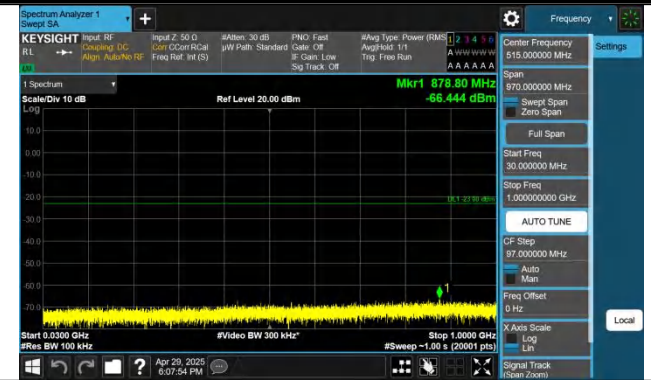
Band2-20MHz-QPSK-19100-1RB#99-30~1000-PASS
