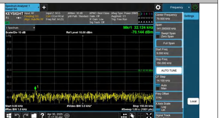
Band2-3MHz-QPSK-19185-1RB#14-0.009~0.15-PASS
