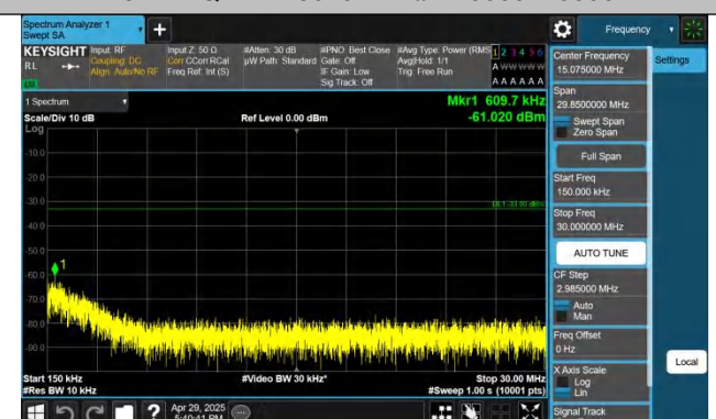
Band2-5MHz-QPSK-18900-1RB#0-0.15~30-PASS
