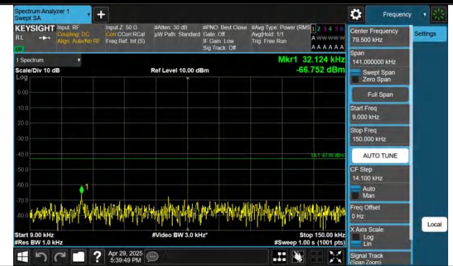
Band2-5MHz-QPSK-18625-1RB#24-0.009~0.15-PASS
