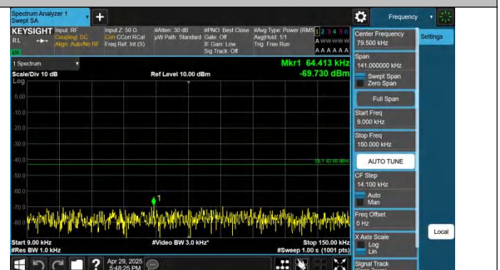
Band2-10MHz-QPSK-18650-1RB#49-0.009~0.15-PASS
