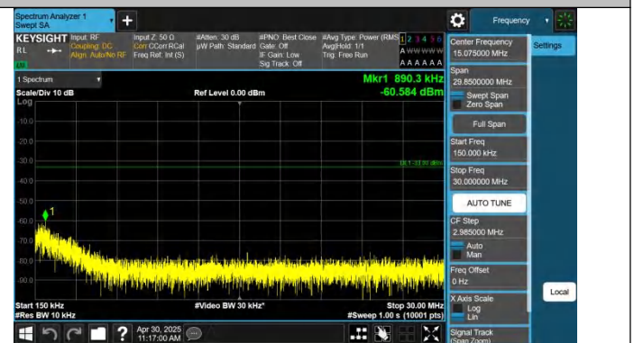
Band2-3MHz-QPSK-19185-1RB#0-0.15~30-PASS
