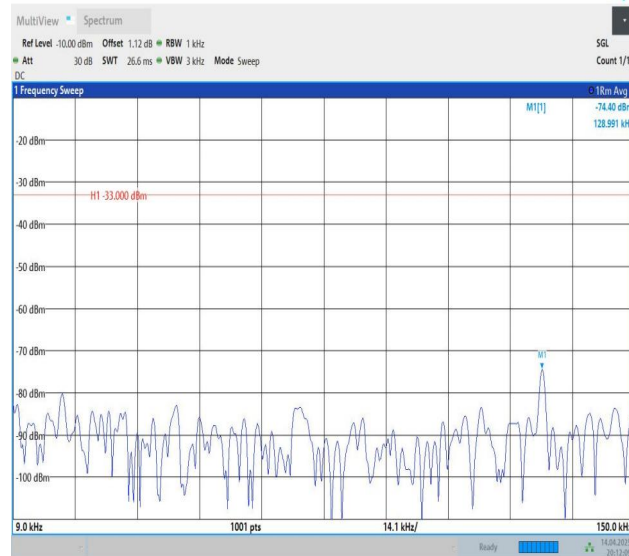
Band12-1.4MHz-QPSK-23173-1RB#5-0.009~0.15-PASS
