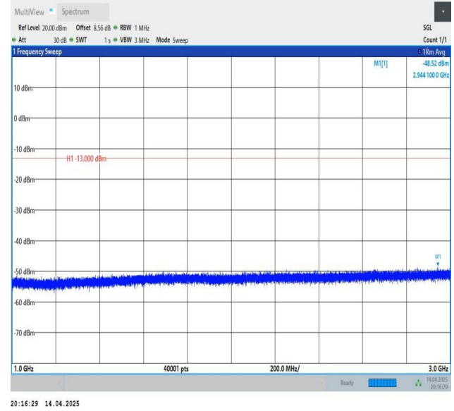
Band12-5MHz-QPSK-23095-1RB#0-1000~3000-PASS
