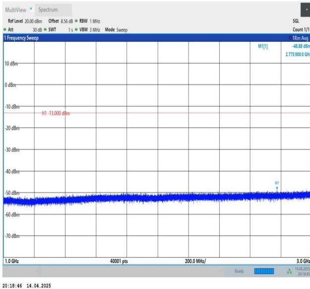
Band12-10MHz-QPSK-23060-1RB#49-1000~3000-PASS
