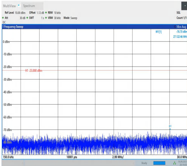
Band12-3MHz-QPSK-23095-1RB#14-0.15~30-PASS
