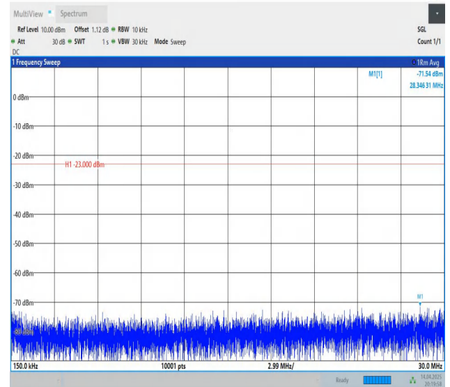
Band12-10MHz-QPSK-23130-1RB#0-0.15~30-PASS
