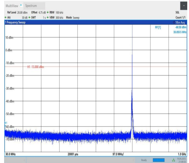
Band12-3MHz-QPSK-23095-1RB#14-30~1000-PASS
