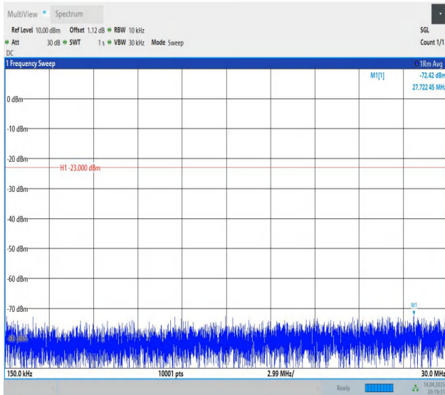
Band12-10MHz-QPSK-23095-1RB#49-0.15~30-PASS
