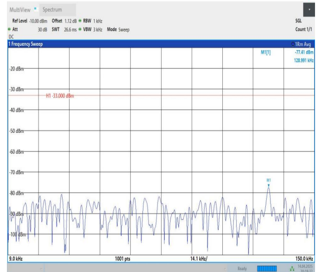
Band12-10MHz-QPSK-23060-1RB#49-0.009~0.15-PASS
