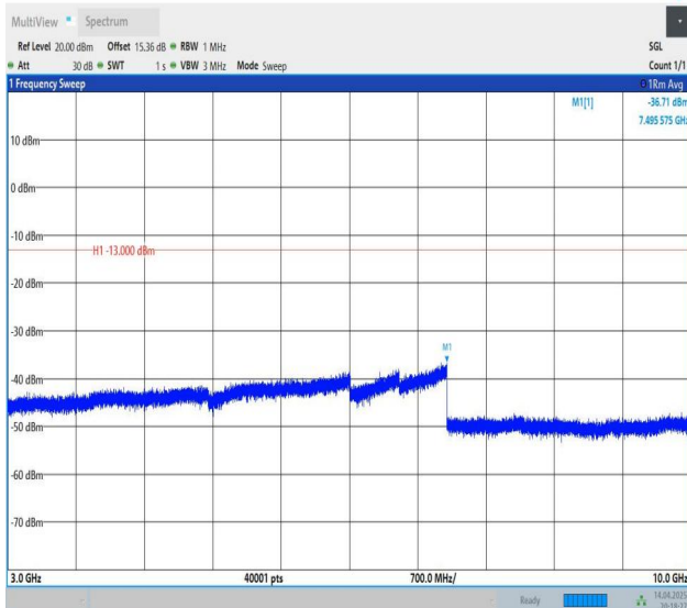
Band12-10MHz-QPSK-23060-1RB#0-3000~10000-PASS
