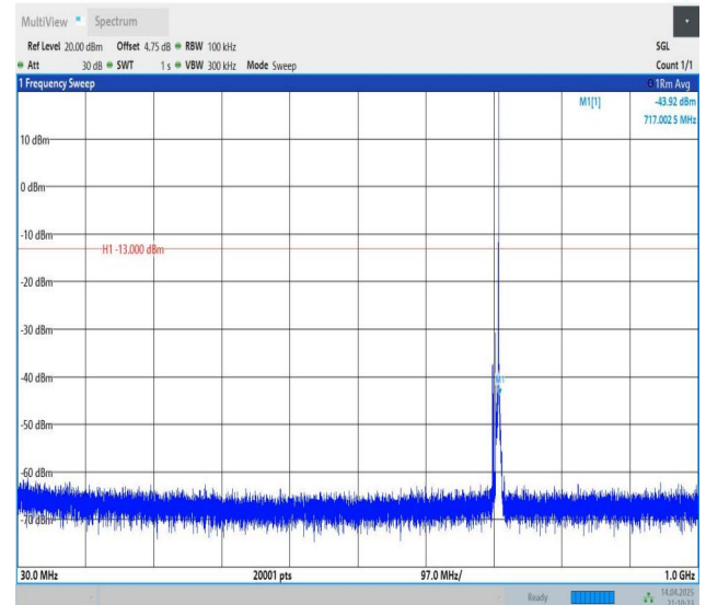
Band12-5MHz-QPSK-23155-1RB#24-30~1000-PASS
