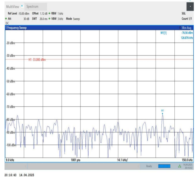
Band12-5MHz-QPSK-23095-1RB#24-0.009~0.15-PASS
