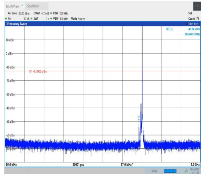
Band12-10MHz-QPSK-23095-1RB#49-30~1000-PASS
