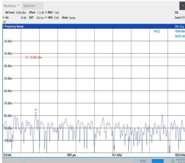
Band12-5MHz-QPSK-23095-1RB#0-0.009~0.15-PASS
