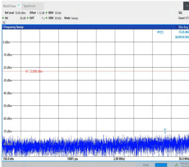
Band12-5MHz-QPSK-23155-1RB#24-0.15~30-PASS
