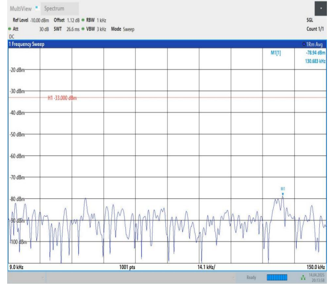
Band12-3MHz-QPSK-23095-1RB#14-0.009~0.15-PASS
