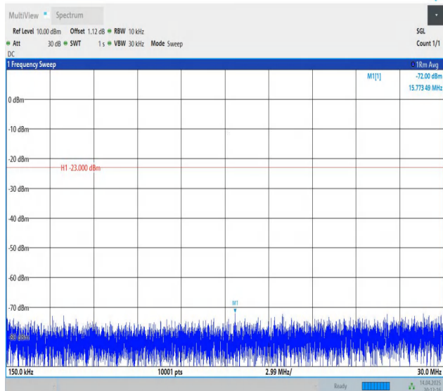
Band12-1.4MHz-QPSK-23173-1RB#5-0.15~30-PASS
