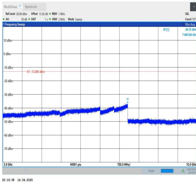
Band12-5MHz-QPSK-23095-1RB#0-3000~10000-PASS
