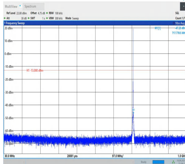
Band12-1.4MHz-QPSK-23173-1RB#5-30~1000-PASS
