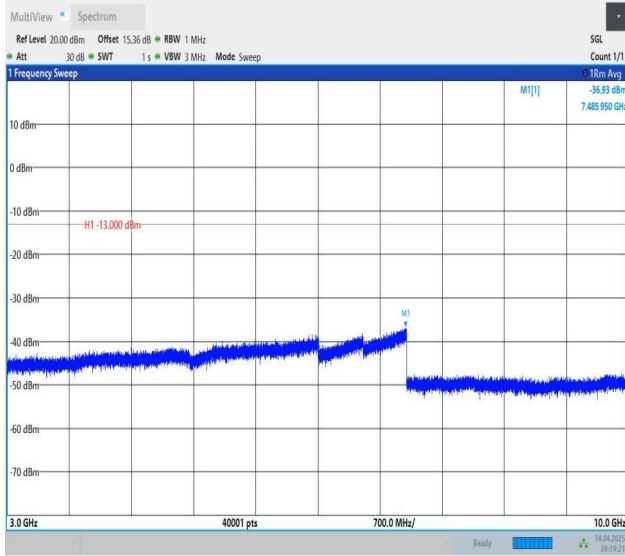
Band12-10MHz-QPSK-23095-1RB#0-3000~10000-PASS
