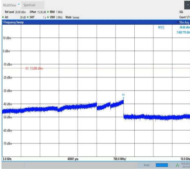
Band12-3MHz-QPSK-23095-1RB#0-3000~10000-PASS
