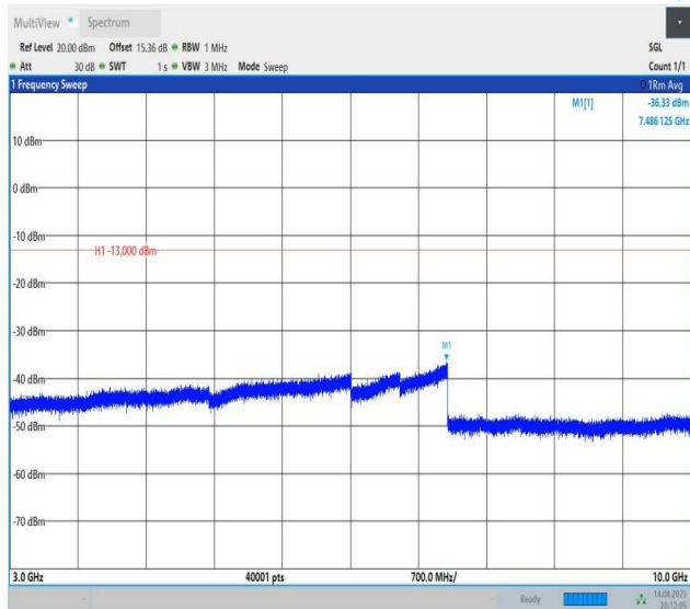
Band12-1.4MHz-QPSK-23173-1RB#0-3000~10000-PASS
