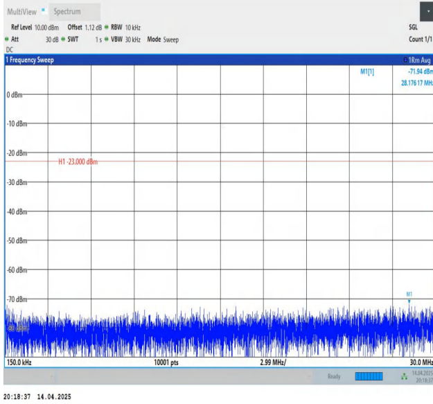
Band12-10MHz-QPSK-23060-1RB#49-0.15~30-PASS
