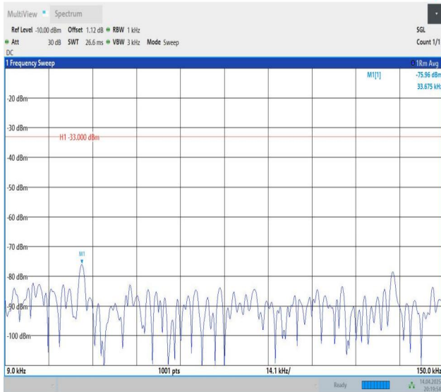
Band12-10MHz-QPSK-23130-1RB#0-0.009~0.15-PASS
