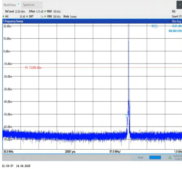
Band12-5MHz-QPSK-23095-1RB#0-30~1000-PASS
