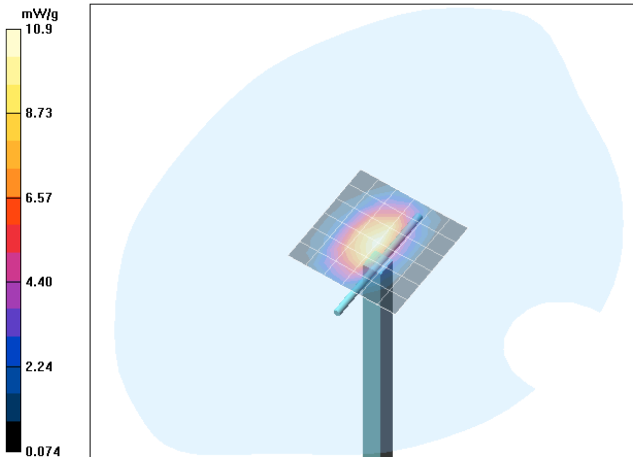
Fig. 12: Validation measurement 1900 MHz body (May 20, 2005), coarse grid. Ambient Temperature: 21.3° C, Liquid Temperature: 20.7° C.
