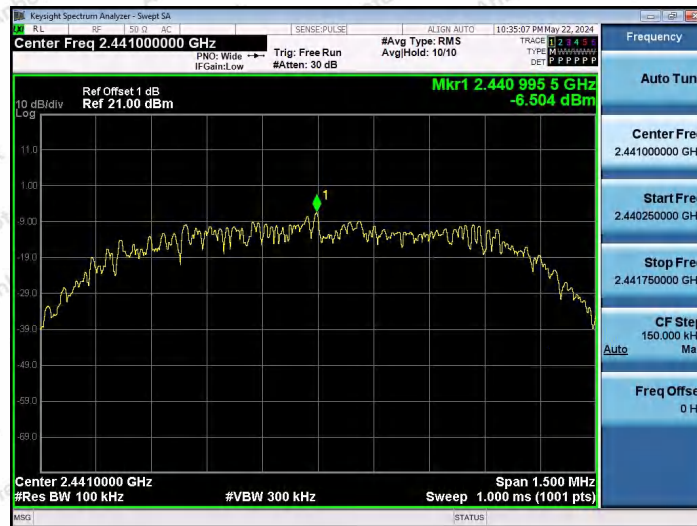
3DH5-Ant1-2441-0~Reference-PASS
