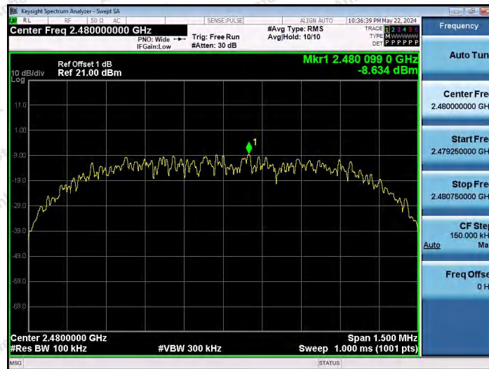
3DH5-Ant1-2480-0~Reference-PASS
