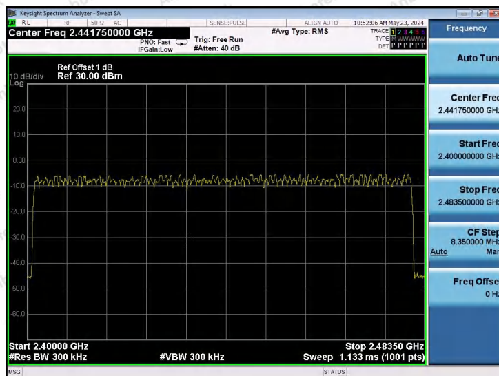
2DH5-Ant1-Hop-PASS
