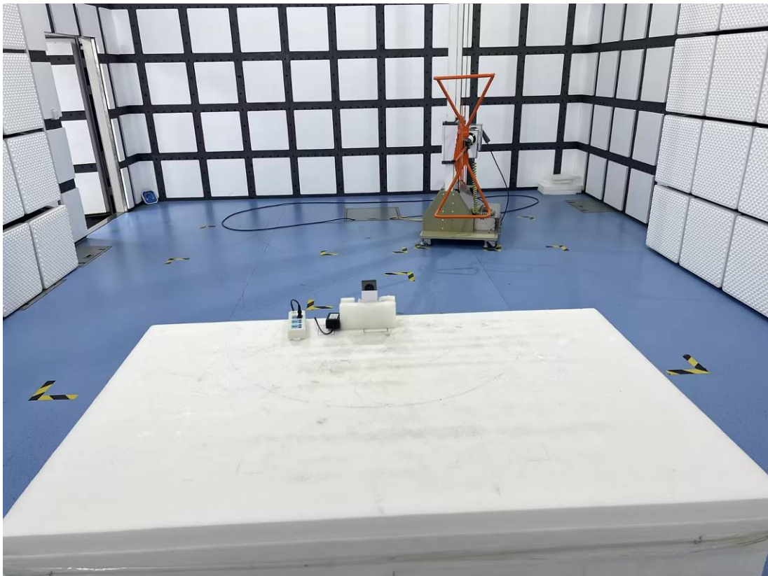
RE-Front View(30MHz~1GHz)(POE)
