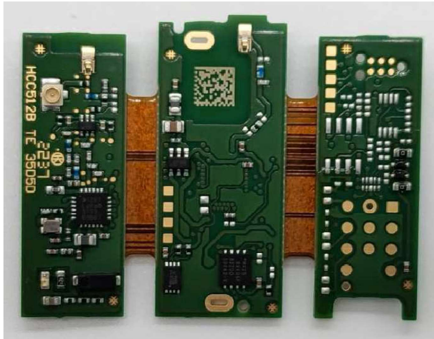
Figure 7. PCB view-1
