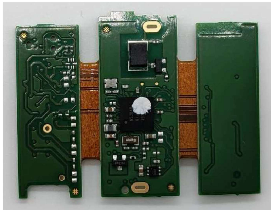
Figure 8. PCB view-2
