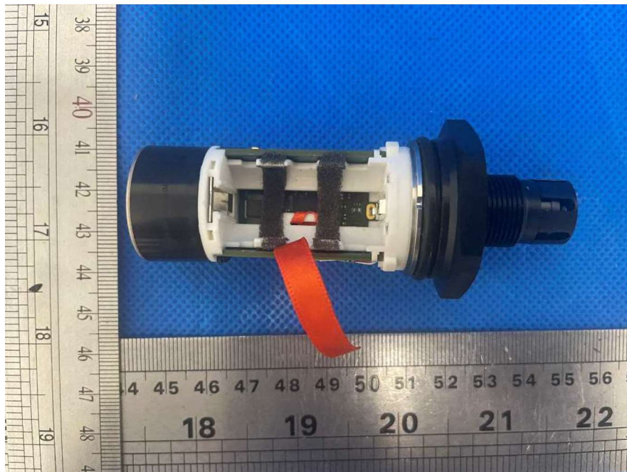
Figure 6. Internal view-3
