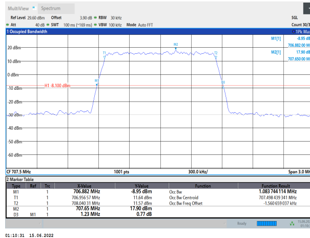
Band12-1.4MHz-QPSK-23095-6RB#0
