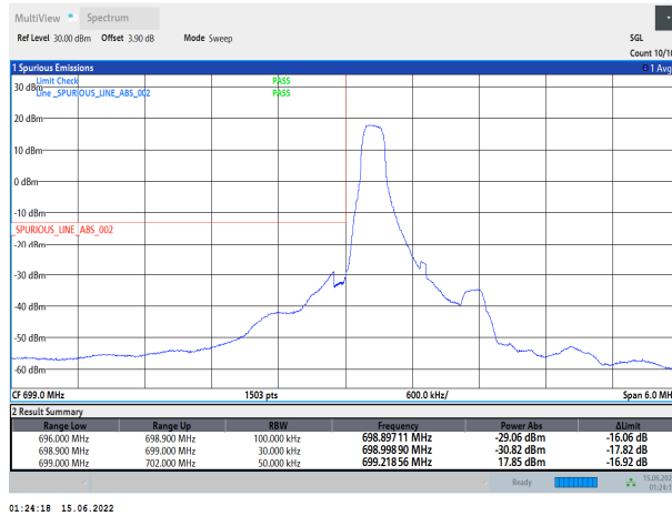
Band12-1.4MHz-QPSK-23017-6RB#0
