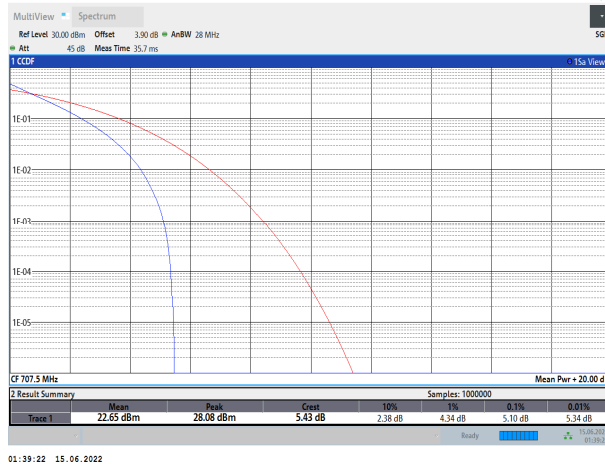
Band12-10MHz-QPSK-23095-50RB#0
