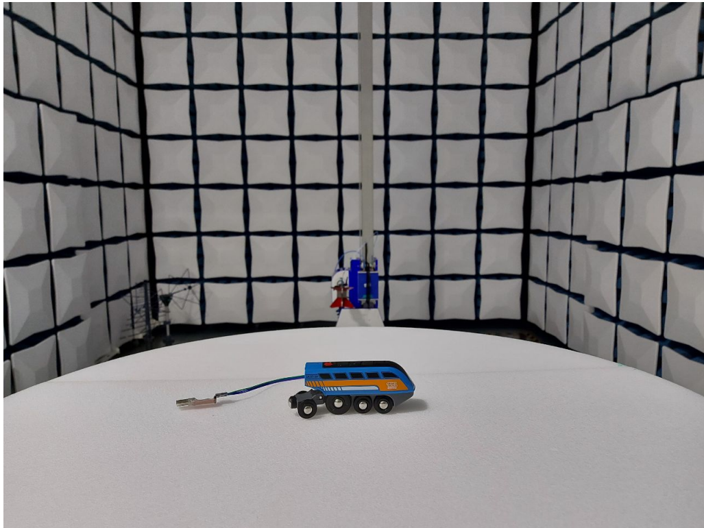
Set-up for Radiated Emission (Model: 3971)
