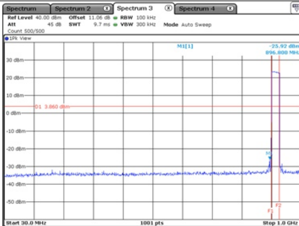
Hopping Channel
