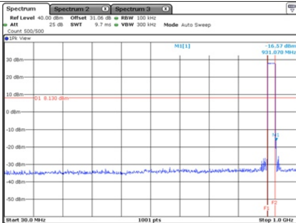
Hopping Channel
