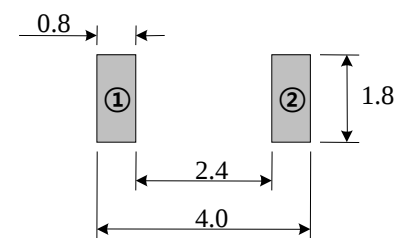
[PCB Solder Land]
