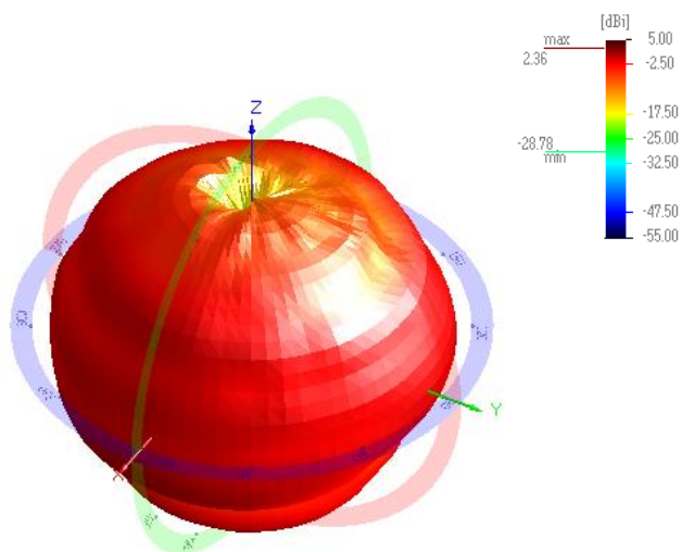
[3D Radiation Pattern @2450MHz]
