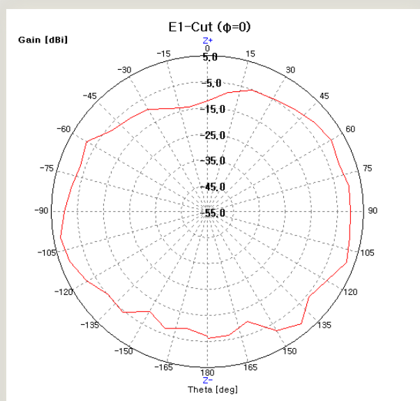
[Elevation1 plane @2.45GHz ]
