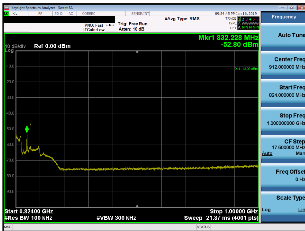
Plot 7-25. Conducted Spurious Plot (LTE Band 26, 10MHz QPSK – RB Size 1, RB Offset 0 – Mid Channel)
