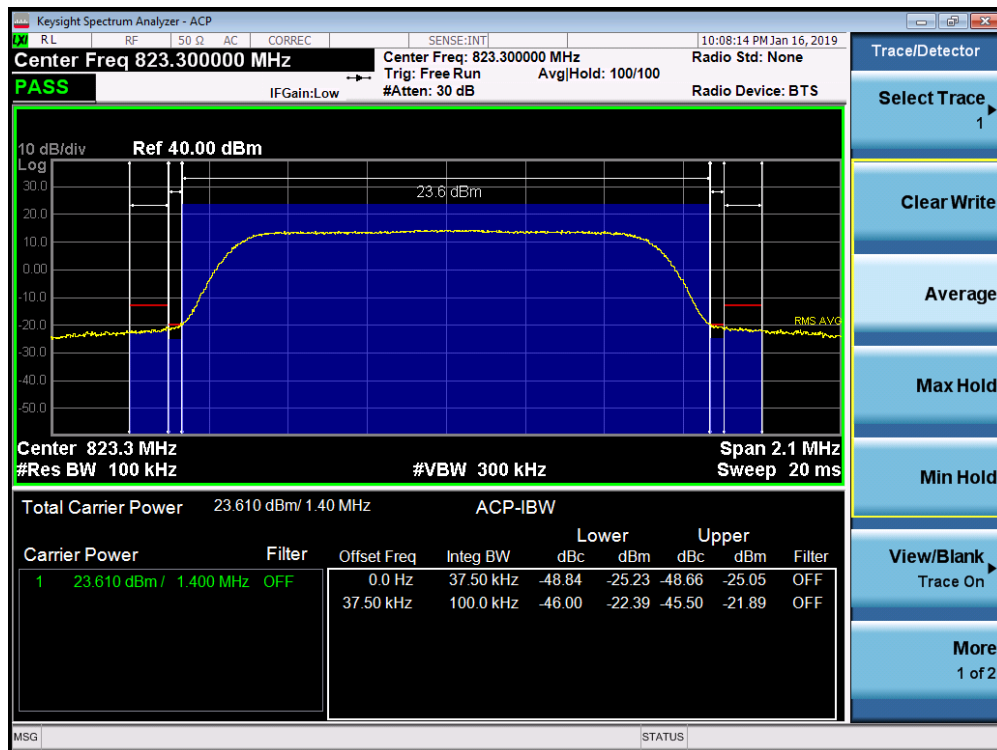
Plot 7-31. Channel Edge Plot (LTE Band 26, 1.4MHz QPSK – RB Size 6 – High Channel)
