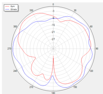
Phi=90 freq=2400MHz
