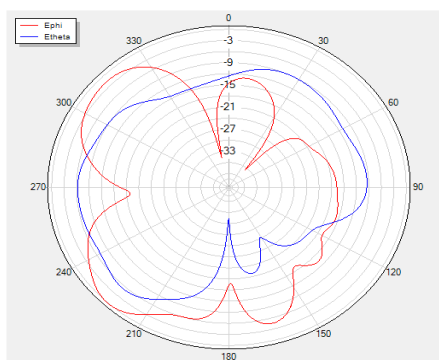
Phi=0 freq=2400MHz
