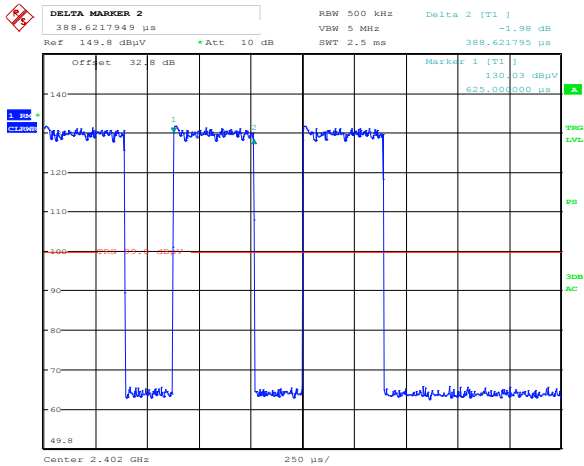
Figure 8.4-3: Radiated spurious emission, band edge, low channel
