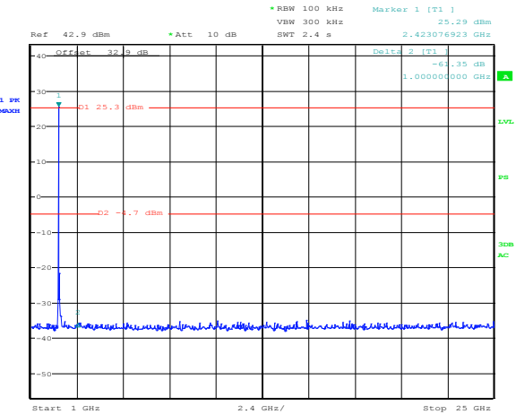
Figure 8.4-8: Conducted spurious, Low channel
