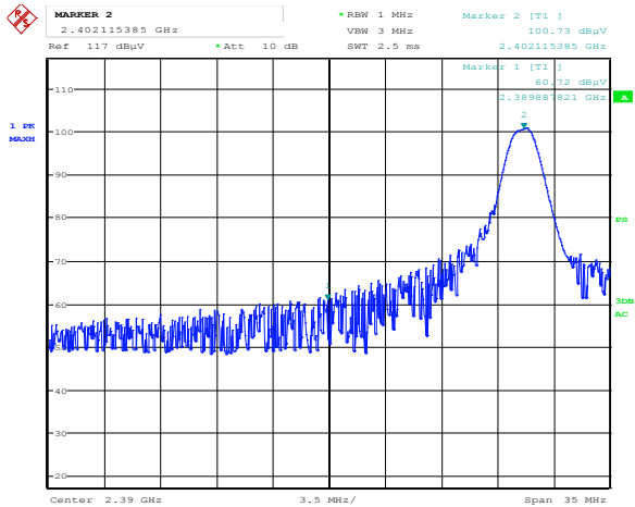
Figure 8.4-1: Conducted spurious emission, low channel
