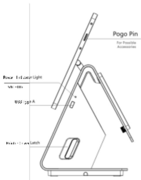
Figure 2: Left view
