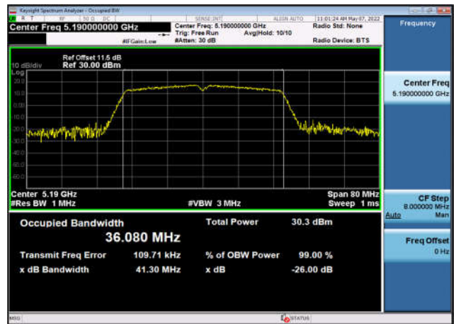
U-NII-1 Occupied Bandwidth-802.11ac(40MHz) ,5190MHz,Ant0
