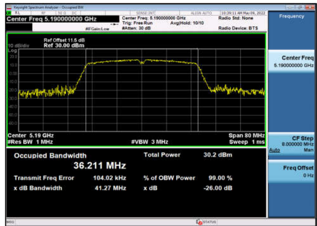
U-NII-1 Occupied Bandwidth-802.11ac(40MHz) ,5190MHz,Ant3
