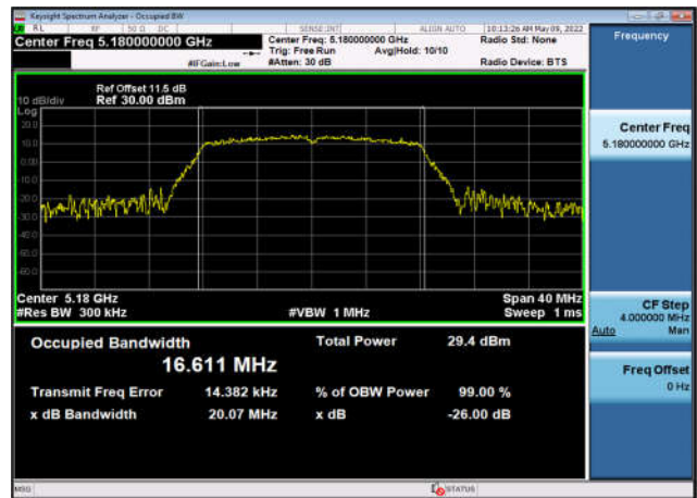
U-NII-1 Occupied Bandwidth-802.11a(20MHz) ,5180MHz,Ant3
