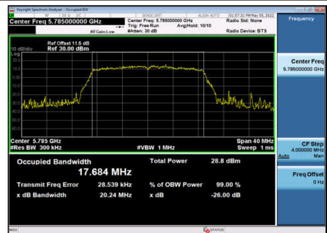
U-NII-3 Occupied Bandwidth -802.11ac(20MHz) ,5785MHz,Ant0
