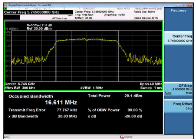
U-NII-3 Occupied Bandwidth-802.11a(20MHz) ,5745MHz,Ant2
