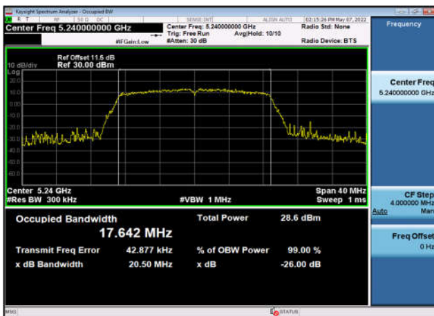
U-NII-1 Occupied Bandwidth-802.11ax(20MHz) ,5240MHz,Ant0
