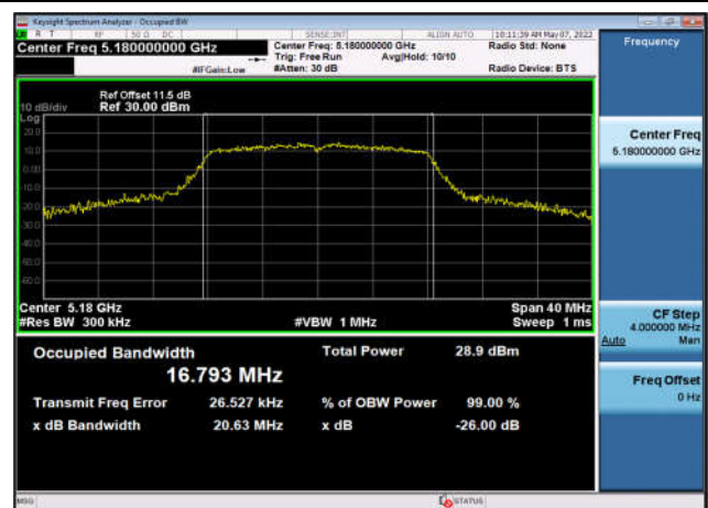
U-NII-1 Occupied Bandwidth-802.11a(20MHz) ,5180MHz,Ant0
