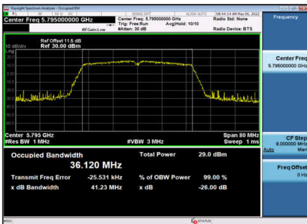
U-NII-3 Occupied Bandwidth-802.11n(40MHz) ,5795MHz,Ant2
