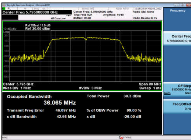
U-NII-3 Occupied Bandwidth -802.11ax(40MHz) ,5795MHz,Ant1
