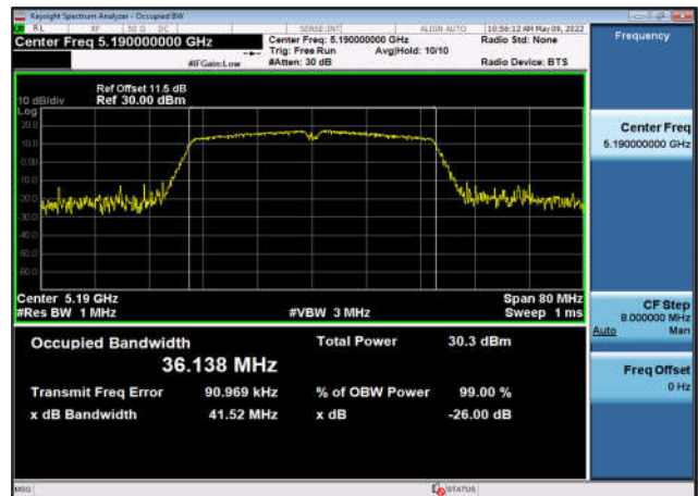
U-NII-1 Occupied Bandwidth-802.11ax(40MHz) ,5190MHz,Ant3
