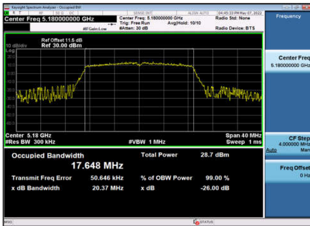
U-NII-1 Occupied Bandwidth-802.11n(20MHz) ,5180MHz,Ant2
