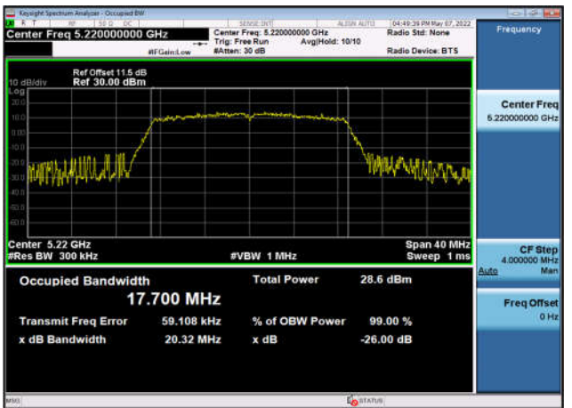
U-NII-1 Occupied Bandwidth-802.11n(20MHz) ,5220MHz,Ant2
