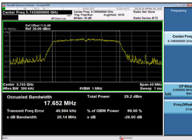
U-NII-3 Occupied Bandwidth -802.11n(20MHz) ,5745MHz,Ant1
