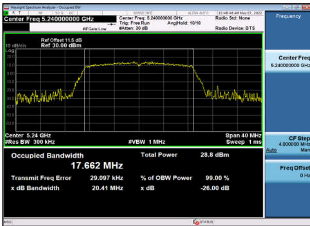
U-NII-1 Occupied Bandwidth-802.11ac(20MHz) ,5240MHz,Ant0
