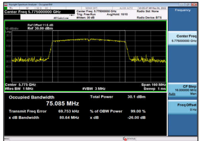
U-NII-3 Occupied Bandwidth-802.11ax(80MHz) ,5775MHz,Ant3
