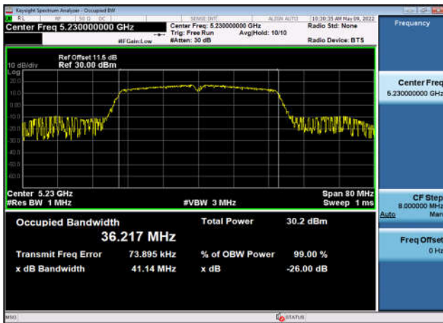
U-NII-1 Occupied Bandwidth-802.11n(40MHz) ,5230MHz,Ant3
