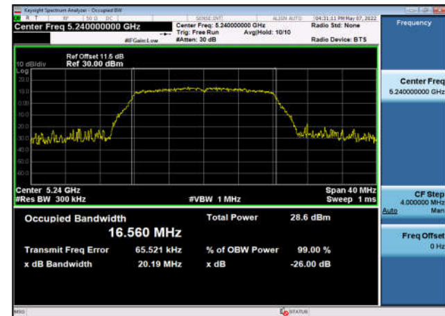
U-NII-1 Occupied Bandwidth-802.11a(20MHz) ,5240MHz,Ant2
