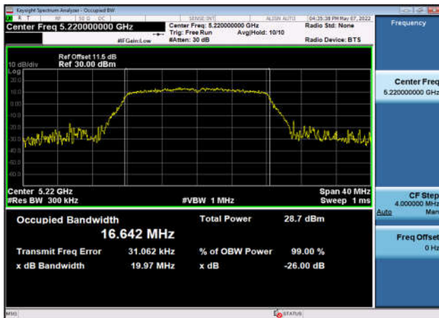
U-NII-1 Occupied Bandwidth-802.11a(20MHz) ,5220MHz,Ant2
