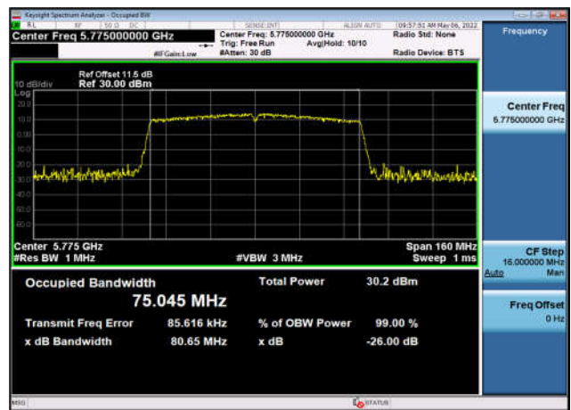
U-NII-3 Occupied Bandwidth -802.11ax(80MHz) ,5775MHz,Ant1
