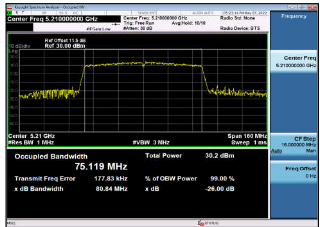
U-NII-1 Occupied Bandwidth-802.11ac(80MHz) ,5210MHz,Ant2
