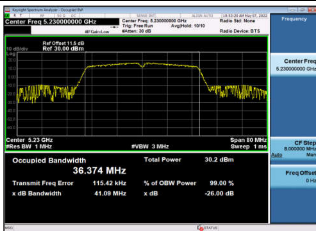
U-NII-1 Occupied Bandwidth-802.11n(40MHz) ,5230MHz,Ant0
