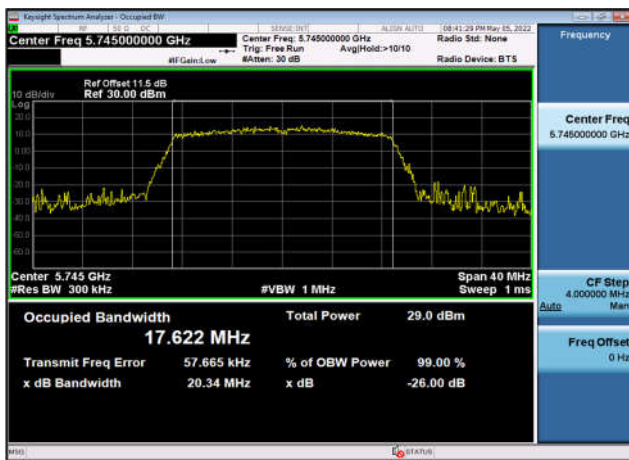
U-NII-3 Occupied Bandwidth-802.11ac(20MHz) ,5745MHz,Ant3
