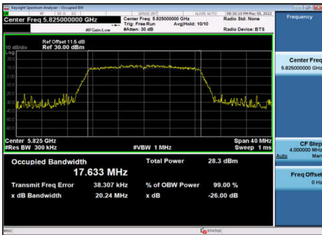
U-NII-3 Occupied Bandwidth-802.11n(20MHz) ,5825MHz,Ant3
