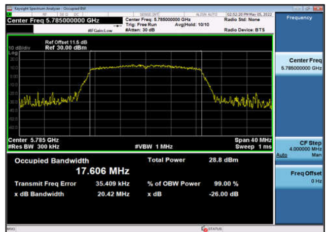
U-NII-3 Occupied Bandwidth-802.11ax(20MHz) ,5785MHz,Ant3
