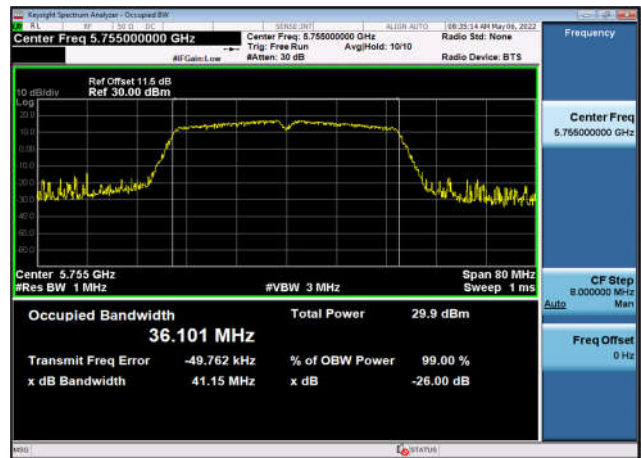
U-NII-3 Occupied Bandwidth-802.11ac(40MHz) ,5755MHz,Ant2
