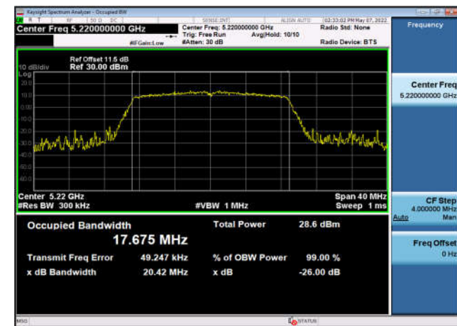
U-NII-1 Occupied Bandwidth-802.11ac(20MHz) ,5220MHz,Ant1
