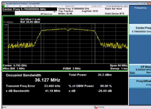
U-NII-3 Occupied Bandwidth-802.11ax(40MHz) ,5795MHz,Ant3
