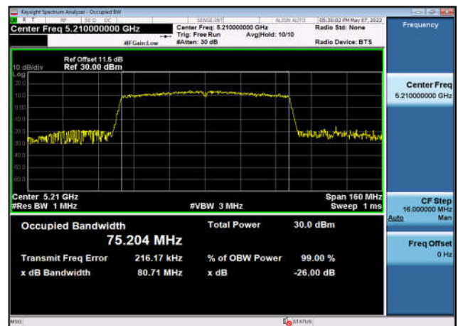
U-NII-1 Occupied Bandwidth-802.11ax(80MHz) ,5210MHz,Ant2
