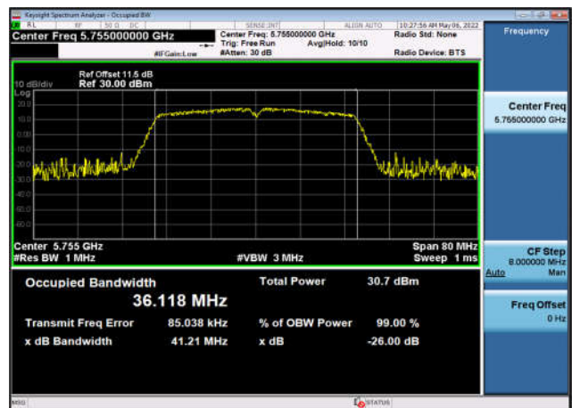
U-NII-3 Occupied Bandwidth-802.11ax(40MHz) ,5755MHz,Ant2
