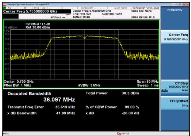
U-NII-3 Occupied Bandwidth-802.11n(40MHz) ,5755MHz,Ant3
