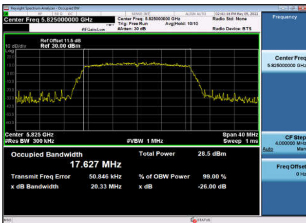
U-NII-3 Occupied Bandwidth-802.11ax(20MHz) ,5825MHz,Ant2
