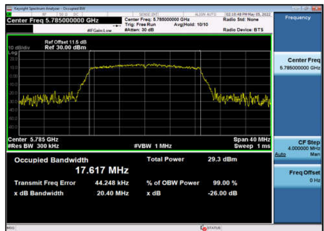
U-NII-3 Occupied Bandwidth -802.11ax(20MHz) ,5785MHz,Ant0
