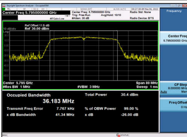
U-NII-3 Occupied Bandwidth -802.11ac(40MHz) ,5795MHz,Ant1
