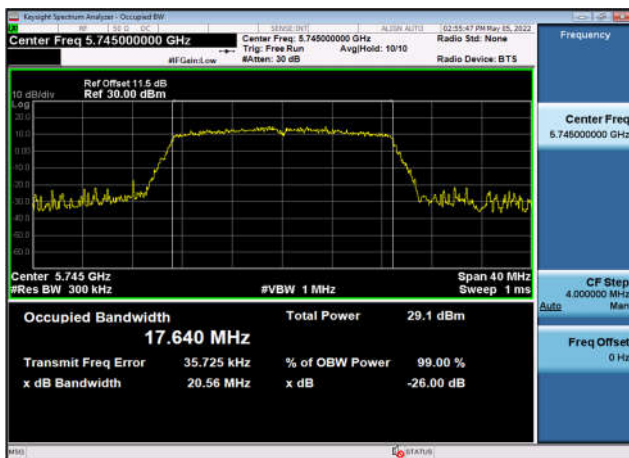
U-NII-3 Occupied Bandwidth-802.11ax(20MHz) ,5745MHz,Ant3
