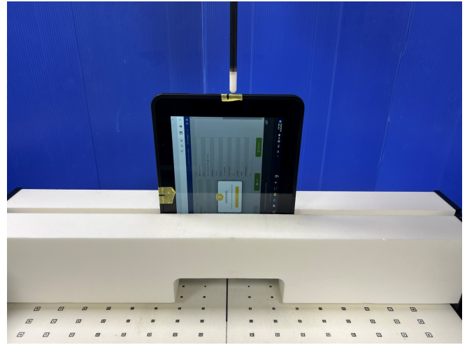
Photo 8: Power Density Right Side_2mm
