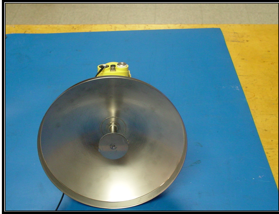
Photograph 37: 33 dBi Parabolic Antenna Front View
