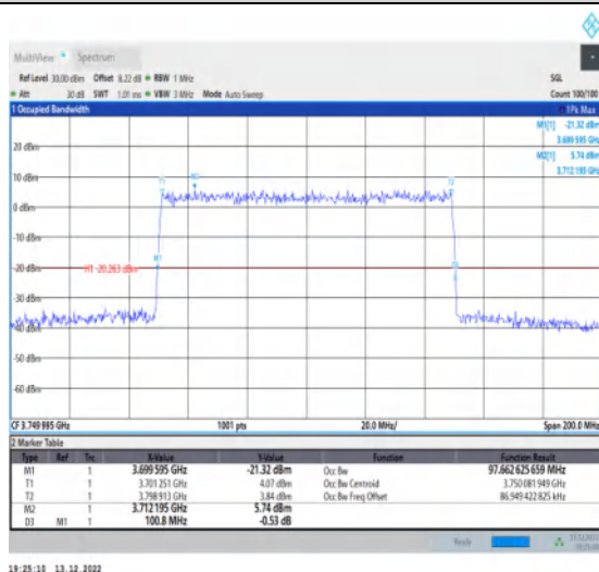
1-N77-3700-3980-30-100-L-9-CP-256QAM-Outer_Full -273@0-Ant1-97.663-100.800≤100-PASS
