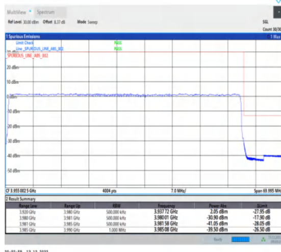
1-N77-3700-3980-30-60-H-3-DFT-PI2BPSK-Outer _Full-162@0-Ant1-1--PASS-see graph
