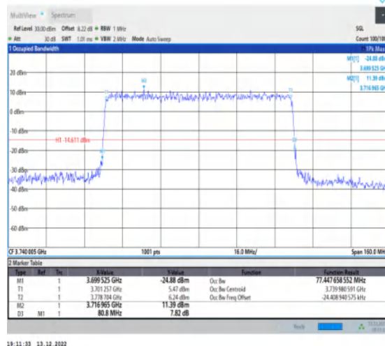
1-N77-3700-3980-30-80-L-6-CP-QPSK-Outer_Full-2 17@0-Ant1-77.448-80.800-≤80-PASS
