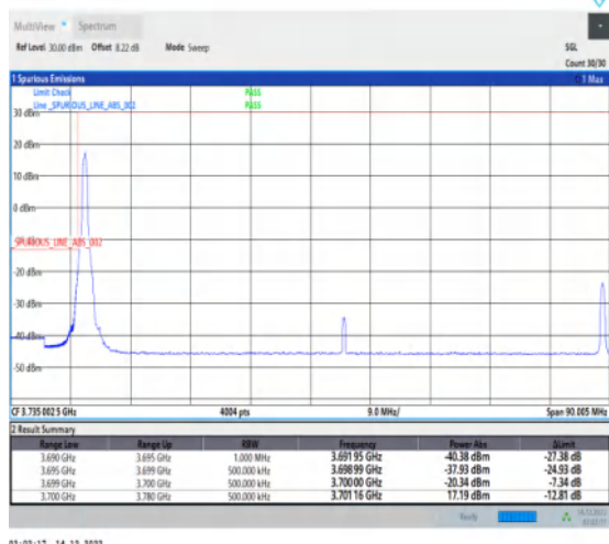
1-N77-3700-3980-30-80-L-4-CP-QPSK-Edge_1RB_Lef t-1@0-Ant1-1--PASS-see graph
