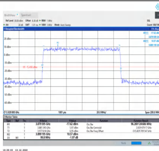
1-N77-3700-3980-30-100-H-4-DFT-64QAM-Outet_Full -270@0-Ant1-96.269-99.800-≤100-PASS
