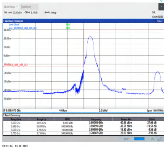
1-N77-3700-3980-30-10-L-1-DFT-PI2BPSK-Edge_1RB_Left-1@0-Ant1-1--PASS-see graph
