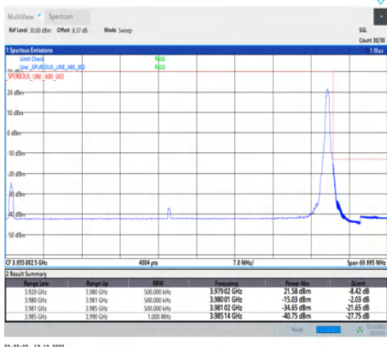
1-N77-3700-3980-30-60-H-2-DFT-PI2BPSK-Edge_1R B_Right-1@161-Ant1-1--PASS-see graph
