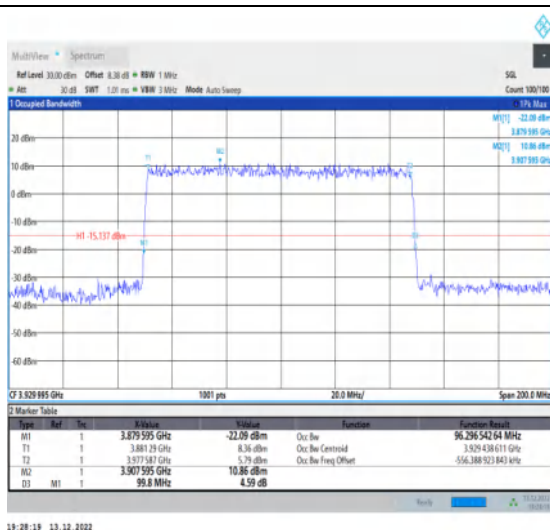
1-N77-3700-3980-30-100-H-1-DFT-QPSK-Outet_Full -270@0-Ant1-96.297-99.800-≤100-PASS
