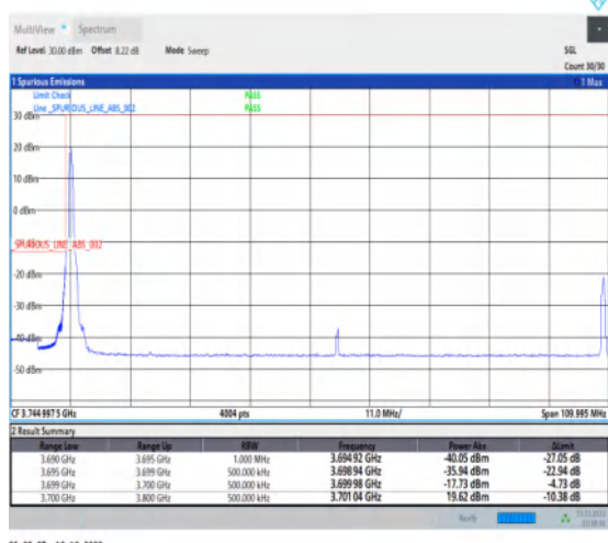
1-N77-3700-3980-30-100-L-4-CP-QPSK-Edge_1RB_Left-1@0-Ant1-1--PASS-see graph
