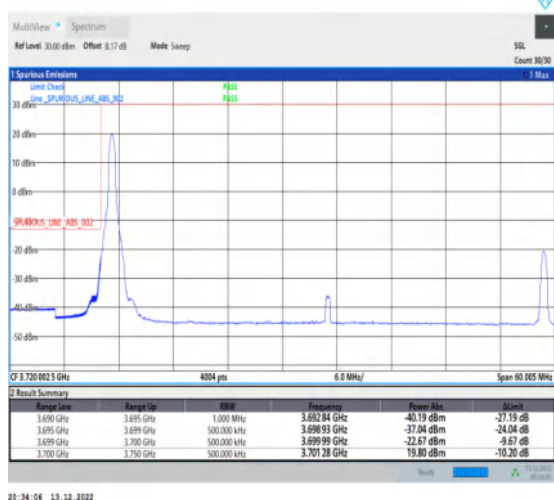
1-N77-3700-3980-30-50-L-4-CP-QPSK-Edge_1RB_Lef t-1@0-Ant1-1--PASS-see graph
