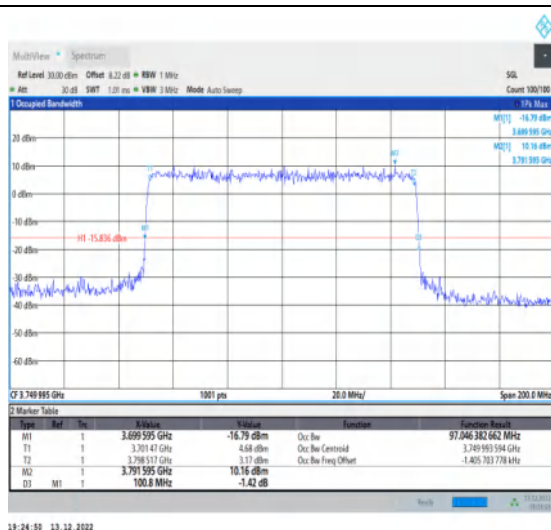
1-N77-3700-3980-30-100-L-7-CP-16QAM-Outer_Full -273@0-Ant1-97.046-100.800≤100-PASS
