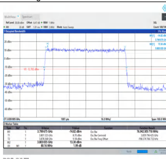
1-N77-3700-3980-30-80-M-1-DFT-QPSK-Outer_Full- 216@0-Ant1-76.942-80.160-≤80-PASS
