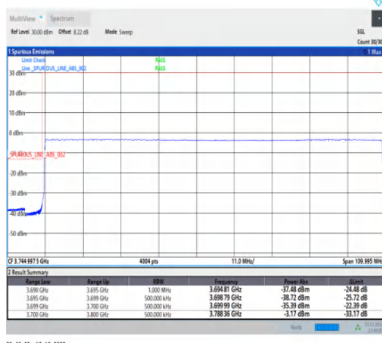
1-N77-3700-3980-30-100-L-6-CP-QPSK-Outer_Full-273@0-Ant1-1--PASS-see graph
