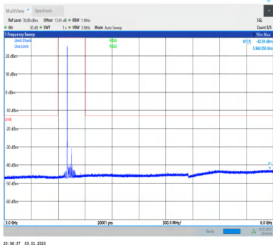
1-N77-3700-3980-30-100-L-1-DFT-QPSK-Edge_1R B_Left-1@0-3000-6000-Ant1-5960.25--42.59--13-PA SS
