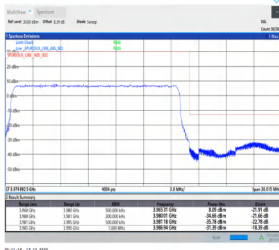
1-N77-3700-3980-30-20-H-3-DFT-PI2BPSK-Outer_Full-50@0-Ant1-1--PASS-see graph
