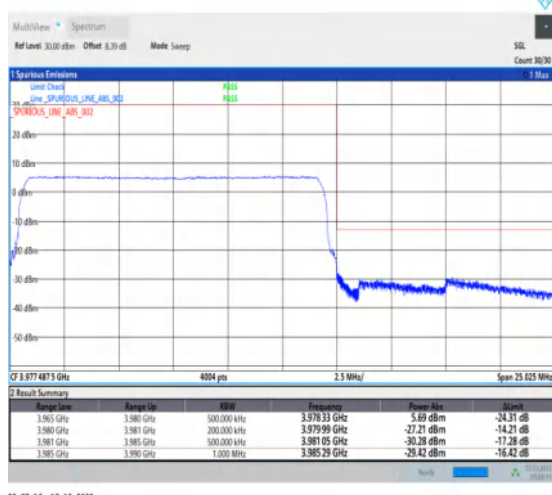
1-N77-3700-3980-30-15-H-6-CP-QPSK-Outer_Full-38@0-Ant1-1--PASS-see graph
