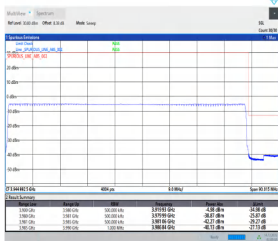
1-N77-3700-3980-30-80-H-6-CP-QPSK-Outer_Full -217@0-Ant1-1--PASS-see graph
