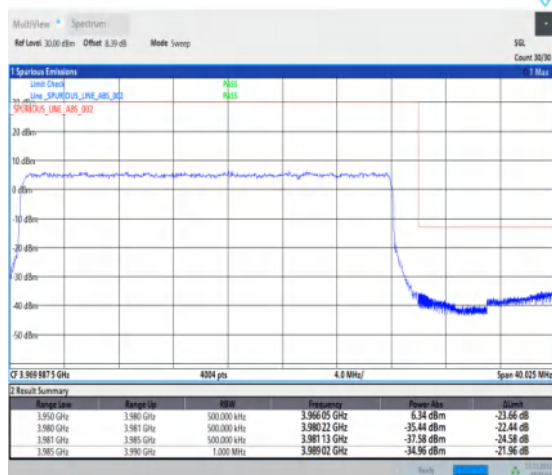
1-N77-3700-3980-30-30-H-3-DFT-PI2BPSK-Outer _Full-75@0-Ant1-1--PASS-see graph
