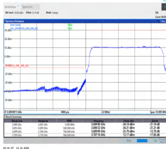
1-N77-3700-3980-30-10-L-3-DFT-PI2BPSK-Outer_Full-24@0-Ant1-1--PASS-see graph
