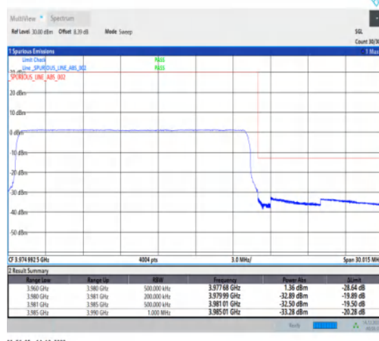
1-N77-3700-3980-30-20-H-6-CP-QPSK-Outer_Full -51@0-Ant1-1--PASS-see graph
