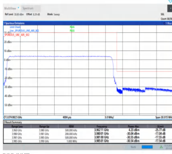
1-N77-3700-3980-30-20-H-6-CP-QPSK-Outer_Full-51@0-Ant1-1--PASS-see graph
