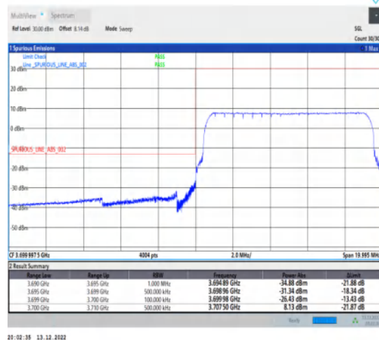
1-N77-3700-3980-30-10-L-6-CP-QPSK-Outer_Full -24@0-Ant1-1--PASS-see graph
