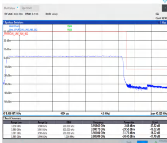
1-N77-3700-3980-30-30-H-6-CP-QPSK-Outer_Full -78@0-Ant1-1--PASS-see graph
