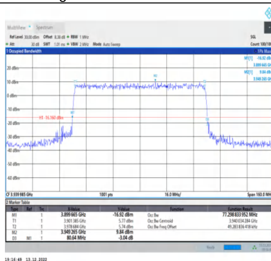
1-N77-3700-3980-30-80-H-8-CP-64QAM-Outer_Full-217@0-Ant1-77.299-80.640-≤80-PASS
