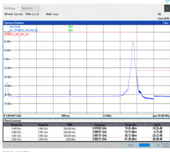
1-N77-3700-3980-30-40-H-5-CP-QPSK-Edge_1RB_Ri ght-1@105-Ant1-1--PASS-see graph
