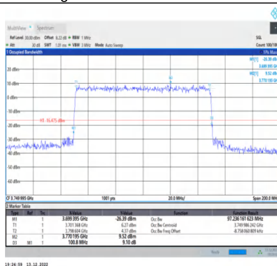
1-N77-3700-3980-30-100-L-8-CP-64QAM-Outer_Full -273@0-Ant1-97.236-100.800≤100-PASS
