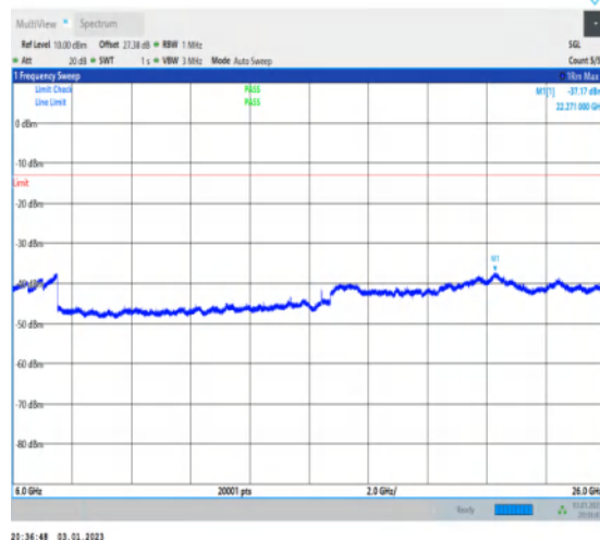
1-N77-3700-3980-30-100-L-1-DFT-QPSK-Edge_1RB _Left-1@0-6000-26000-Ant1-22271.00--37.17--13-P ASS
