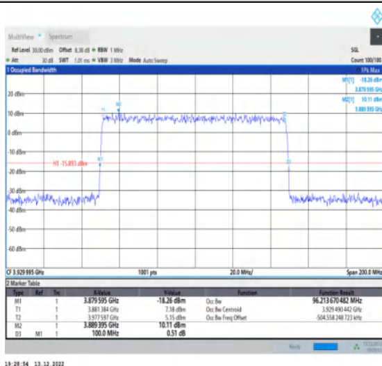
1-N77-3700-3980-30-100-H-3-DFT-16QAM-Outet_Full -270@0-Ant1-96.214-100.000-≤100-PASS
