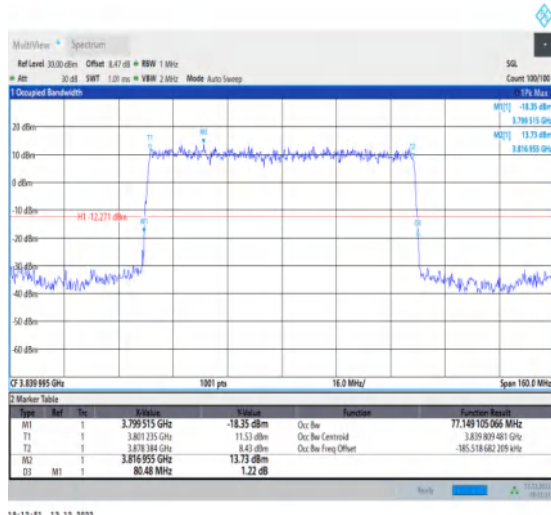
1-N77-3700-3980-30-80-M-2-DFT-PI2BPSK-Outer_F ull-216@0-Ant1-77.149-80.480-≤80-PASS
