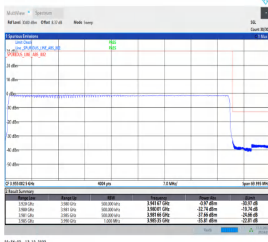
1-N77-3700-3980-30-60-H-6-CP-QPSK-Outer_Full -162@0-Ant1-1--PASS-see graph
