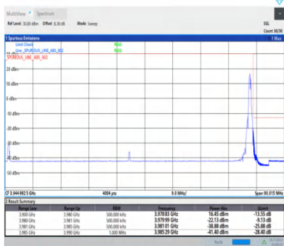
1-N77-3700-3980-30-80-H-5-CP-QPSK-Edge_1RB_Ri ght-1@216-Ant1-1--PASS-see graph
