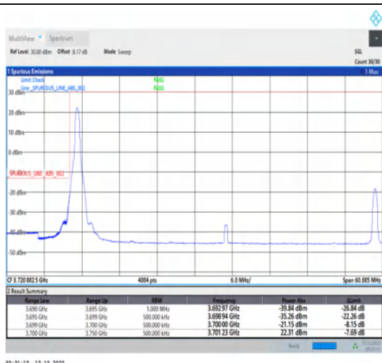
1-N77-3700-3980-30-50-L-1-DFT-PI2BPSK-Edge_1RB_Left-1@0-Ant1-1--PASS-see graph
