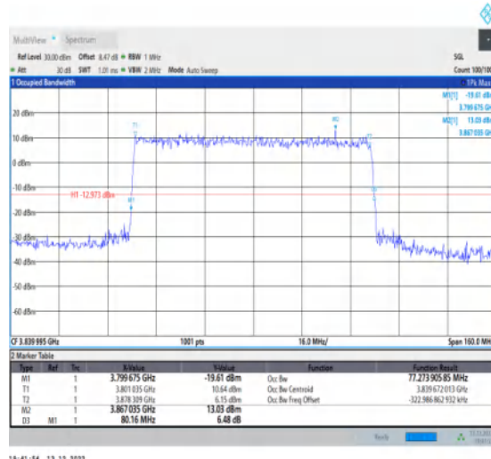
1-N77-3700-3980-30-80-M-3-DFT-16QAM-Outer_Ful l-216@0-Ant1-77.274-80.160-≤80-PASS
