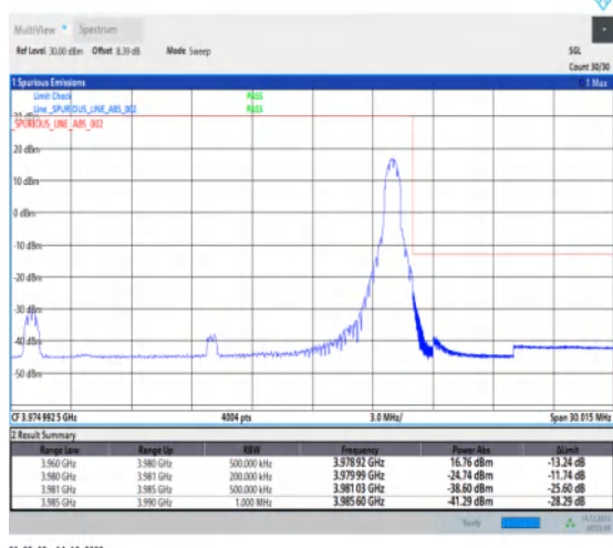
1-N77-3700-3980-30-20-H-5-CP-QPSK-Edge_1RB_Ri ght-1@50-Ant1-1--PASS-see graph
