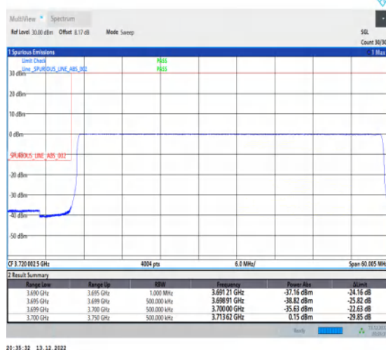
1-N77-3700-3980-30-50-L-6-CP-QPSK-Outer_Full -133@0-Ant1-1--PASS-see graph
