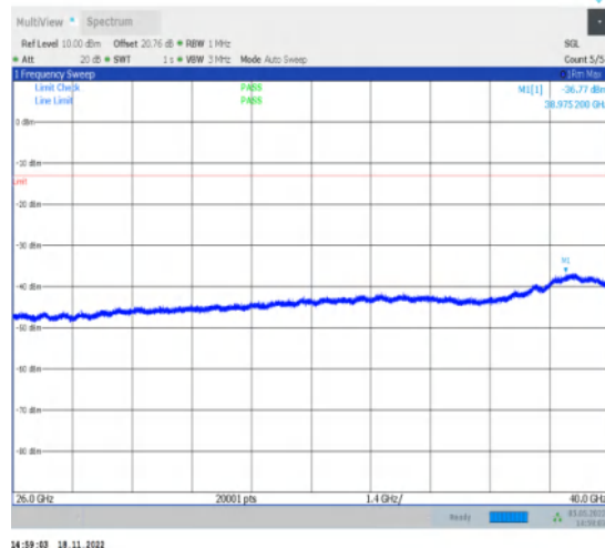
1-N77-3700-3980-30-100-M-1-DFT-QPSK-Edge_1R B_Left-1@0-26000-40000-Ant1-26000.00--42.98--13 -PASS
