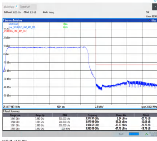
1-N77-3700-3980-30-15-H-3-DFT-PI2BPSK-Outer_Full-36@0-Ant1-1--PASS-see graph
