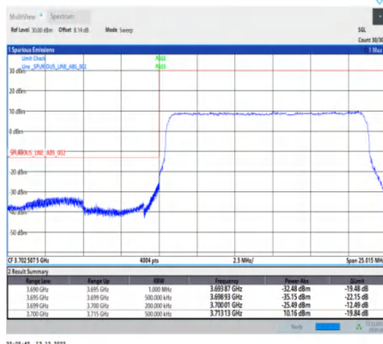
1-N77-3700-3980-30-15-L-3-DFT-PI2BPSK-Outer_Full-36@0-Ant1-1--PASS-see graph
