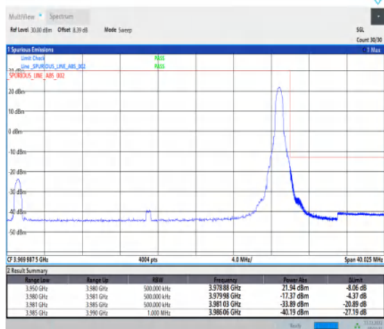
1-N77-3700-3980-30-30-H-2-DFT-PI2BPSK-Edge_1R B_Right-1@77-Ant1-1--PASS-see graph
