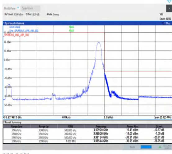
1-N77-3700-3980-30-15-H-5-CP-QPSK-Edge_1RB_Right-1@37-Ant1-1--PASS-see graph
