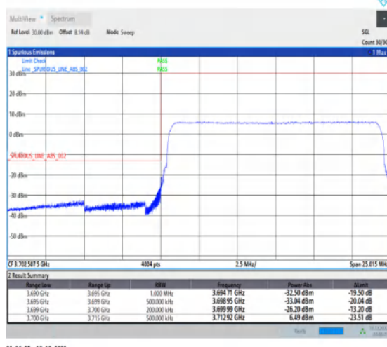
1-N77-3700-3980-30-15-L-6-CP-QPSK-Outer_Full -38@0-Ant1-1--PASS-see graph
