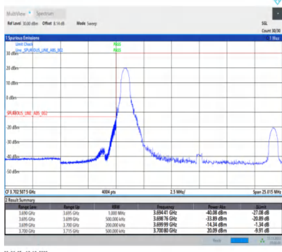
1-N77-3700-3980-30-15-L-4-CP-QPSK-Edge_1RB_Lef t-1@0-Ant1-1--PASS-see graph
