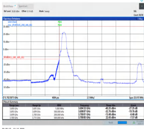
1-N77-3700-3980-30-15-L-1-DFT-PI2BPSK-Edge_1RB_Left-1@0-Ant1-1--PASS-see graph
