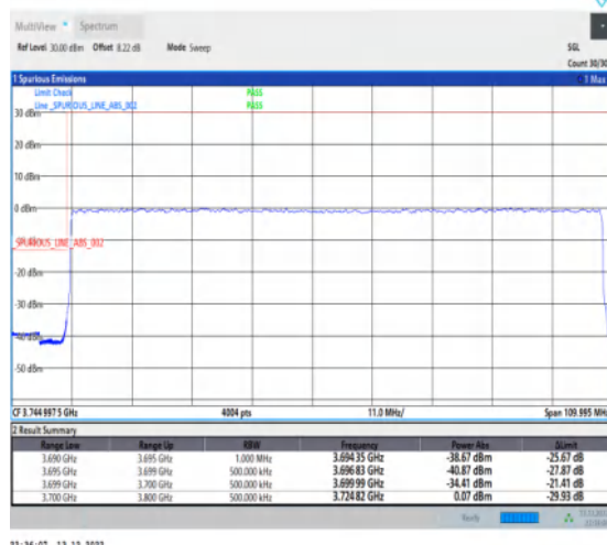
1-N77-3700-3980-30-100-L-3-DFT-PI2BPSK-Outer_Full-270@0-Ant1-1--PASS-see graph
