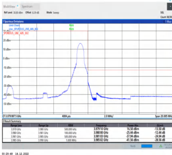
1-N77-3700-3980-30-10-H-5-CP-QPSK-Edge_1RB_Ri ght-1@23-Ant1-1--PASS-see graph
