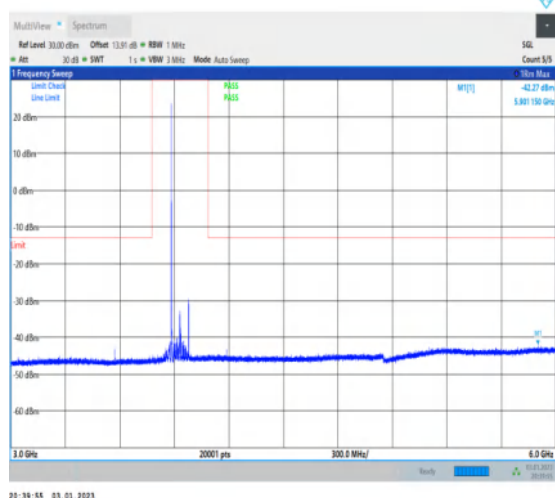
1-N77-3700-3980-30-100-H-1-DFT-QPSK-Edge_1R B_Left-1@0-3000-6000-Ant1-5901.15--42.27--13-PA SS
