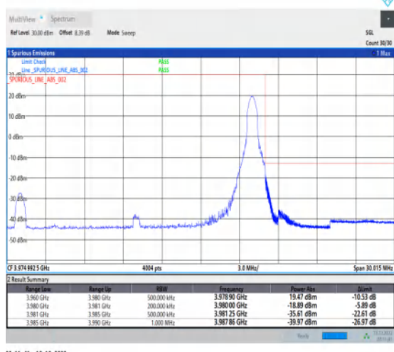
1-N77-3700-3980-30-20-H-5-CP-QPSK-Edge_1RB_Right-1@50-Ant1-1--PASS-see graph
