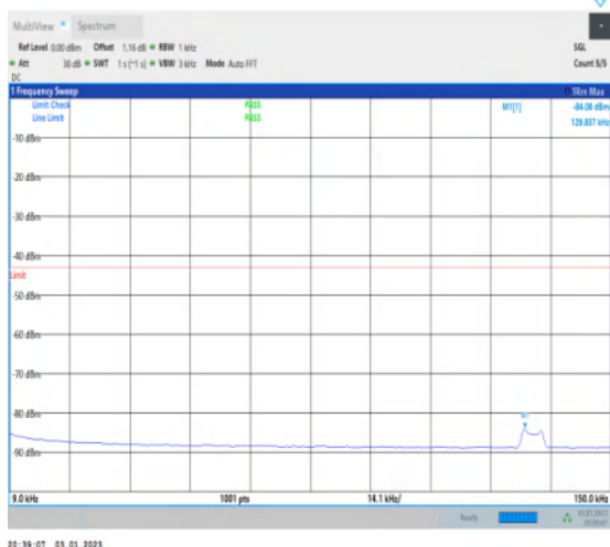
1-N77-3700-3980-30-100-H-1-DFT-QPSK-Edge_1R B_Left-1@0-0.009-0.15-Ant1-0.13--84.08--43-PASS
