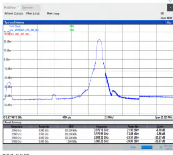
1-N77-3700-3980-30-15-H-2-DFT-PI2BPSK-Edge_1R_B_Right-1@37-Ant1-1--PASS-see graph
