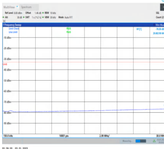
1-N77-3700-3980-30-100-H-1-DFT-QPSK-Edge_1R B_Left-1@0-0.15-30-Ant1-29.80--76.58--33-PASS
