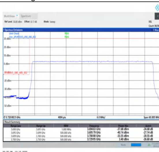
1-N77-3700-3980-30-50-L-3-DFT-PI2BPSK-Outer_Full-128@0-Ant1-1--PASS-see graph
