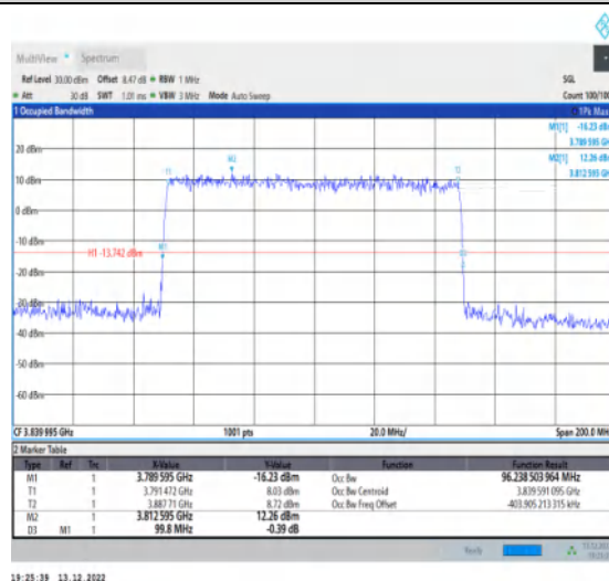
1-N77-3700-3980-30-100-M-1-DFT-QPSK-Outer_Full -270@0-Ant1-96.239-99.800≤100-PASS
