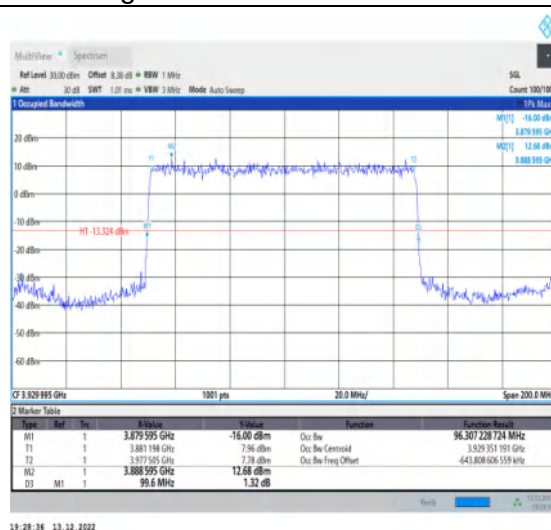
1-N77-3700-3980-30-100-H-2-DFT-PI2BPSK-Outet_Full -270@0-Ant1-96.307-99.600-≤100-PASS
