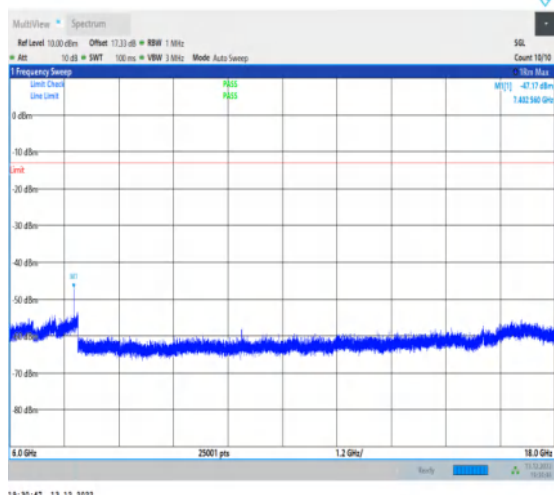
1-N77-3700-3980-30-100-L-1-DFT-PI2BPSK-Inner_1RB_Left-1@1-6000-18000-Ant1-7402.56--47.17--1 3-PASS
