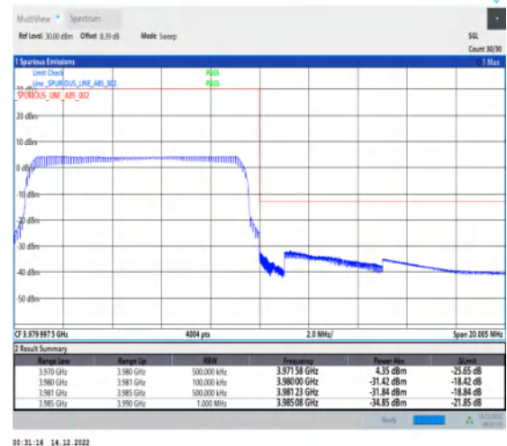
1-N77-3700-3980-30-10-H-6-CP-QPSK-Outer_Full -24@0-Ant1-1--PASS-see graph
