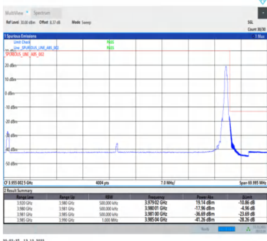
1-N77-3700-3980-30-60-H-5-CP-QPSK-Edge_1RB_Ri ght-1@161-Ant1-1--PASS-see graph
