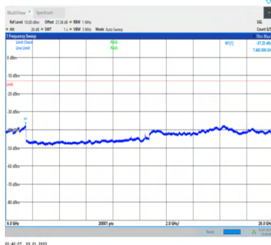
1-N77-3700-3980-30-100-H-1-DFT-QPSK-Edge_1R B_Left-1@0-6000-26000-Ant1-7482.00--37.25--13-P ASS
