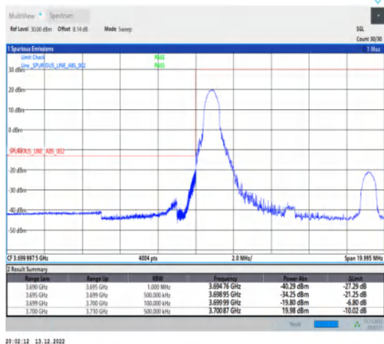
1-N77-3700-3980-30-10-L-4-CP-QPSK-Edge_1RB_Lef t-1@0-Ant1-1--PASS-see graph
