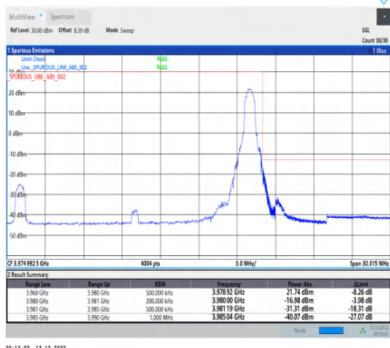
1-N77-3700-3980-30-20-H-2-DFT-PI2BPSK-Edge_1R_B_Right-1@50-Ant1-1--PASS-see graph
