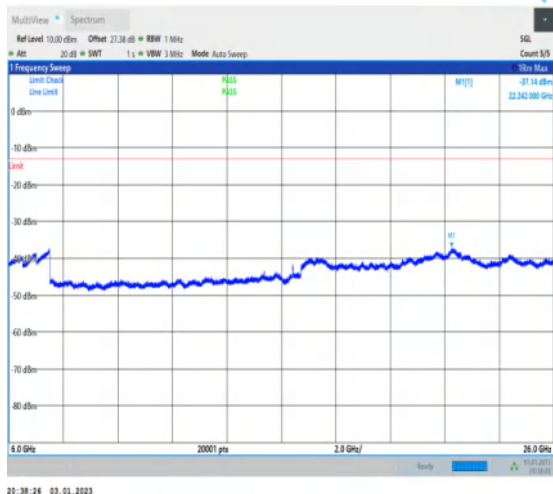
1-N77-3700-3980-30-100-M-1-DFT-QPSK-Edge_1R B_Left-1@0-6000-26000-Ant1-22242.00--37.14--13- PASS
