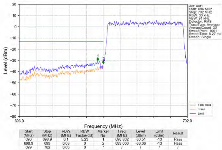
Band12_3MHz_QPSK_LCH_700.5MHz_RB_15_0_NTNV
