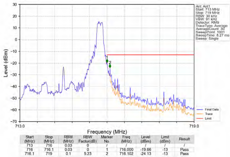
Band12_3MHz_16QAM_HCH_714.5MHz_RB_1_14_NTNV
