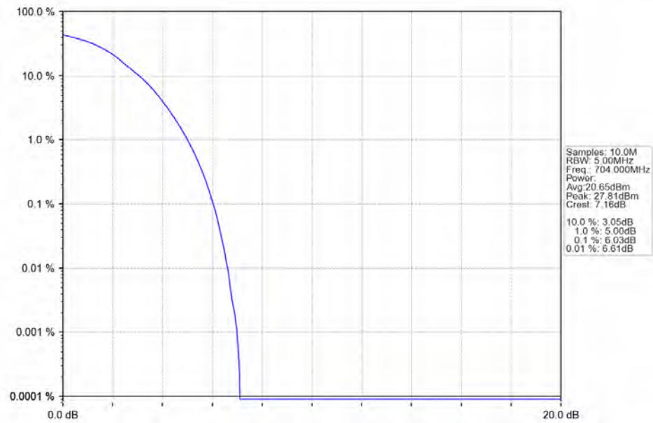
Band12_10MHz_16QAM_LCH_704MHz_RB_50_0_NTNV
