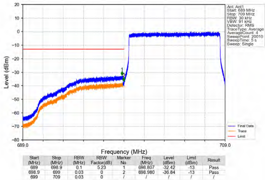
Band12_10MHz_16QAM_LCH_704MHz_RB_50_0_NTNV
