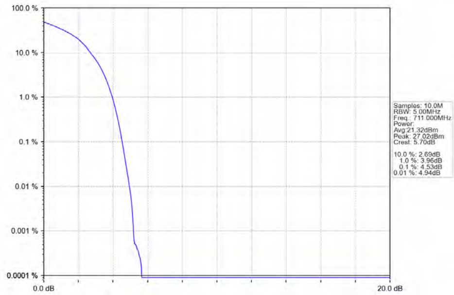
Band12_10MHz_QPSK_HCH_711MHz_RB_50_0_NTNV
