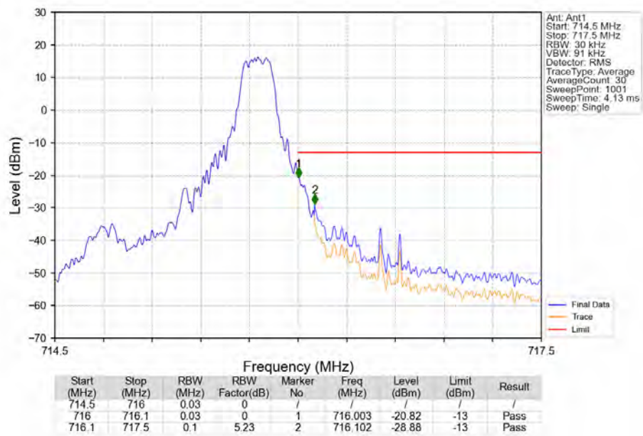
Band12_1.4MHz_QPSK_HCH_715.3MHz_RB_1_5_NTNV
