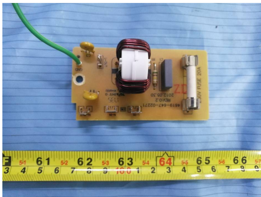
EUT – Filter Circuit Board Top View
