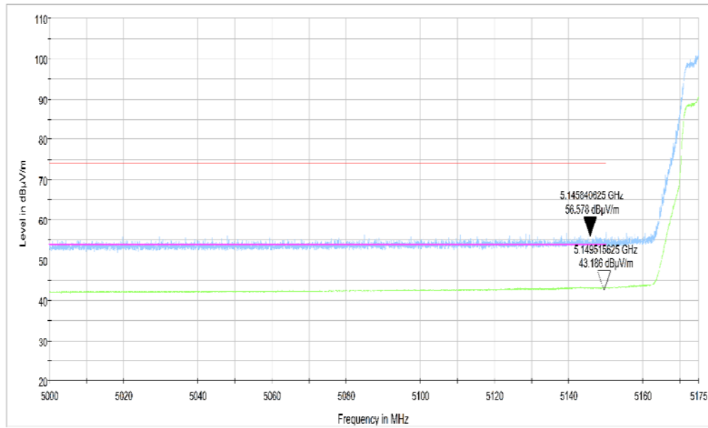
Fig.67 Band Edges (802.11ac-HT20, 5180MHz)
