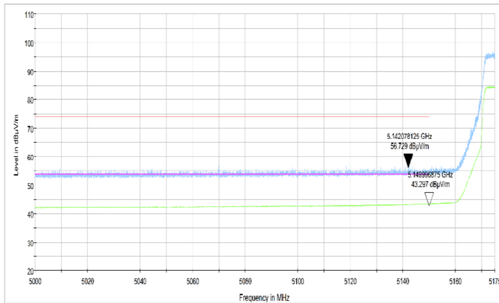
Fig.57 Band Edges (802.11ax-HT40, 5190MHz)
