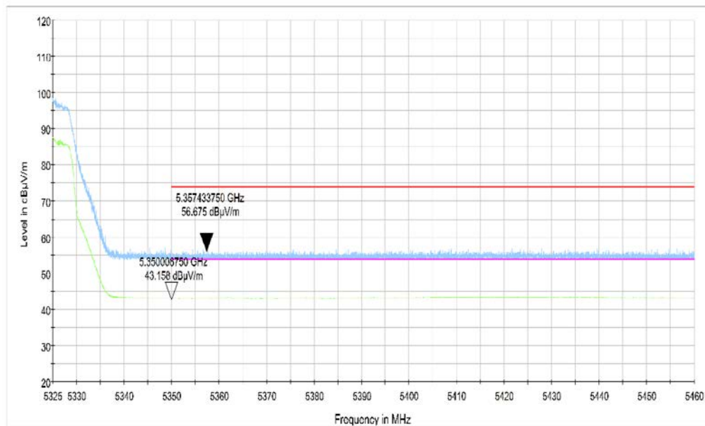
Fig.68 Band Edges (802.11ac-HT20, 5320MHz)
