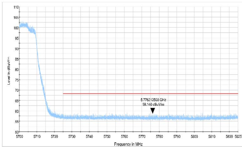
Fig.16 Band Edges (802.11ax-HT20, 5700MHz)
