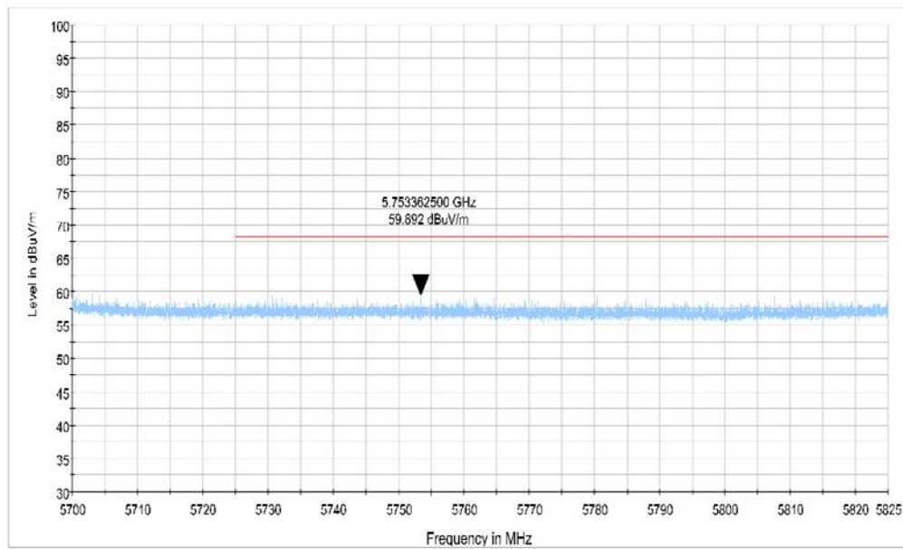
Fig.34 Band Edges (802.11ac-HT40, 5670MHz)
