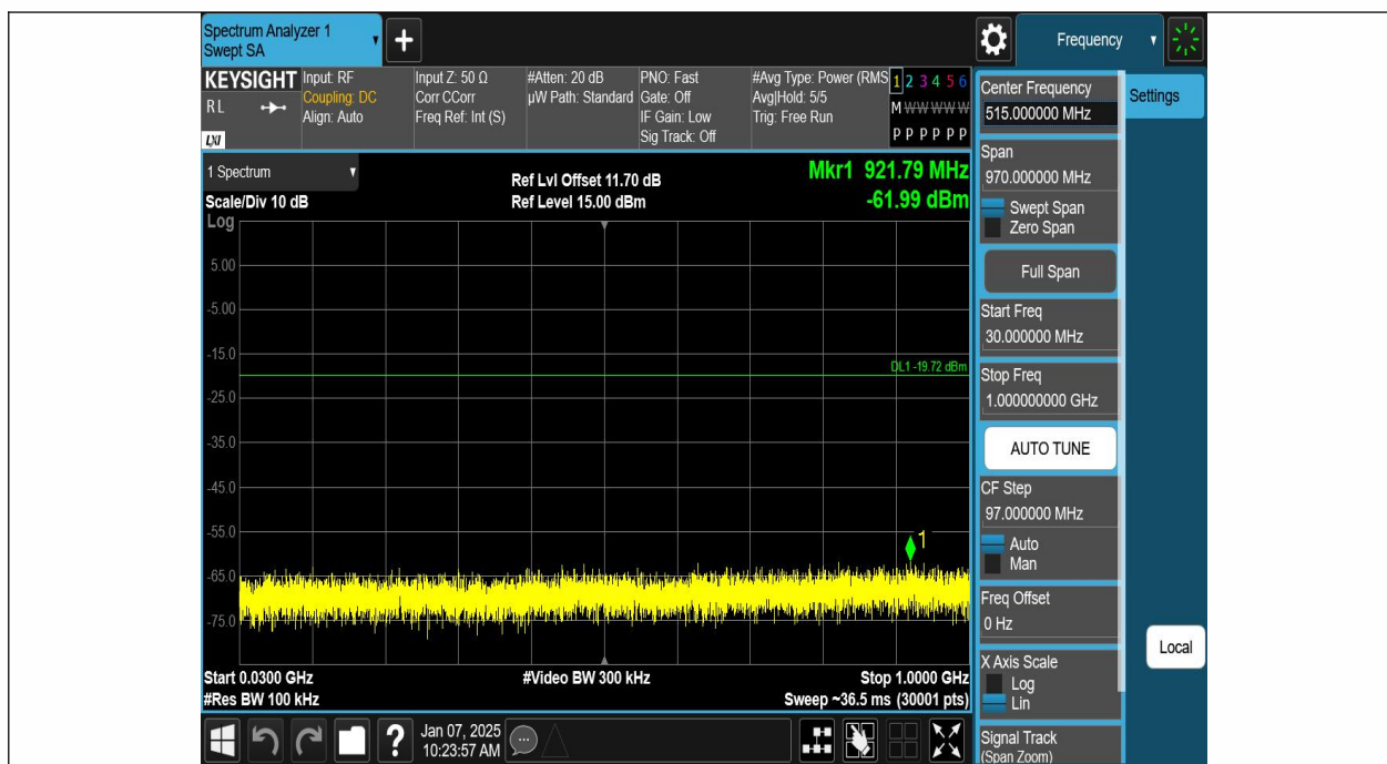
BLE_1M-Ant1-2440-30~1000-PASS
