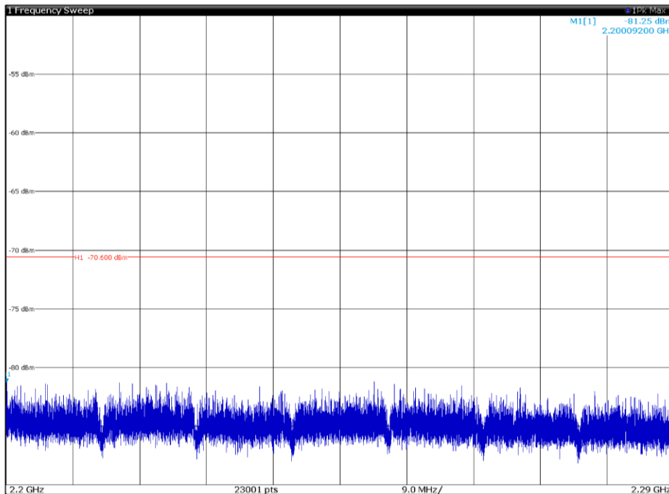
Channel: BOTTOM, Modulation: 64QAM, BW=15MHz, Range: 2200MHz-2290GHz, Polarization: Vertical
