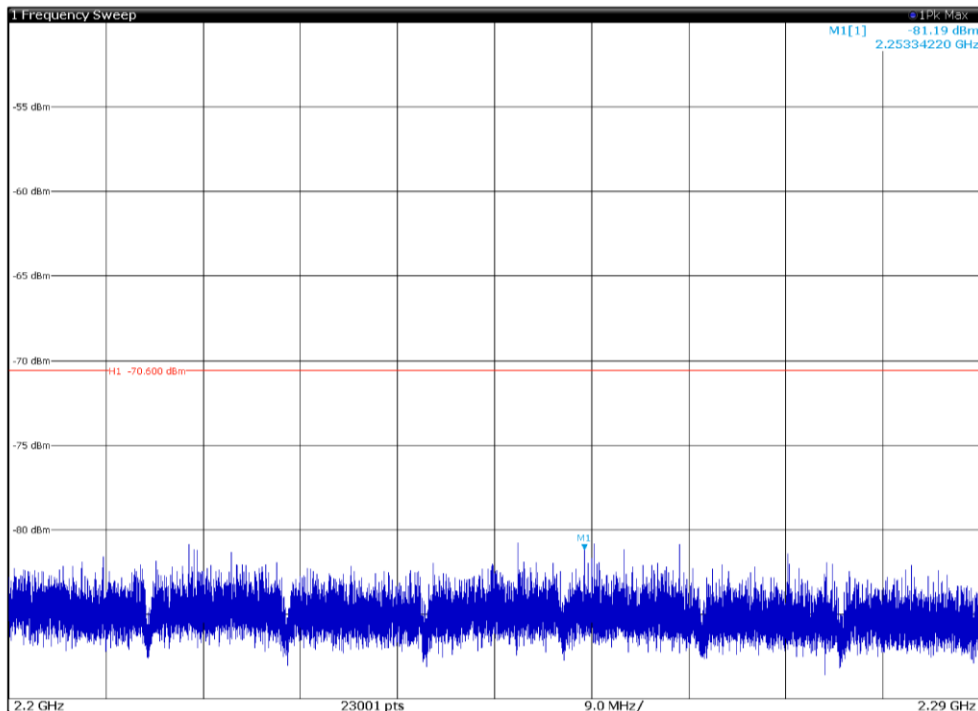
Channel: TOP, Modulation: 16QAM, BW=10MHz, Range: 2200MHz-2290GHz, Polarization: Vertical
