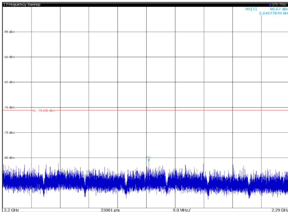
Channel: BOTTOM, Modulation: 256QAM, BW=15MHz, Range: 2200MHz-2290GHz, Polarization: Vertical
