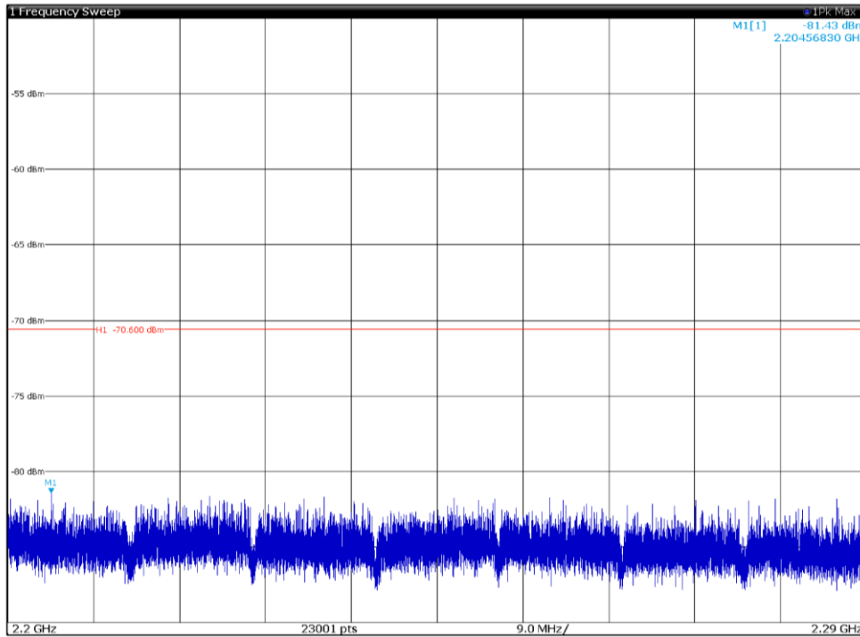
Channel: BOTTOM, Modulation: 256QAM, BW=15MHz, Range: 2200MHz-2290GHz, Polarization: Horizontal
