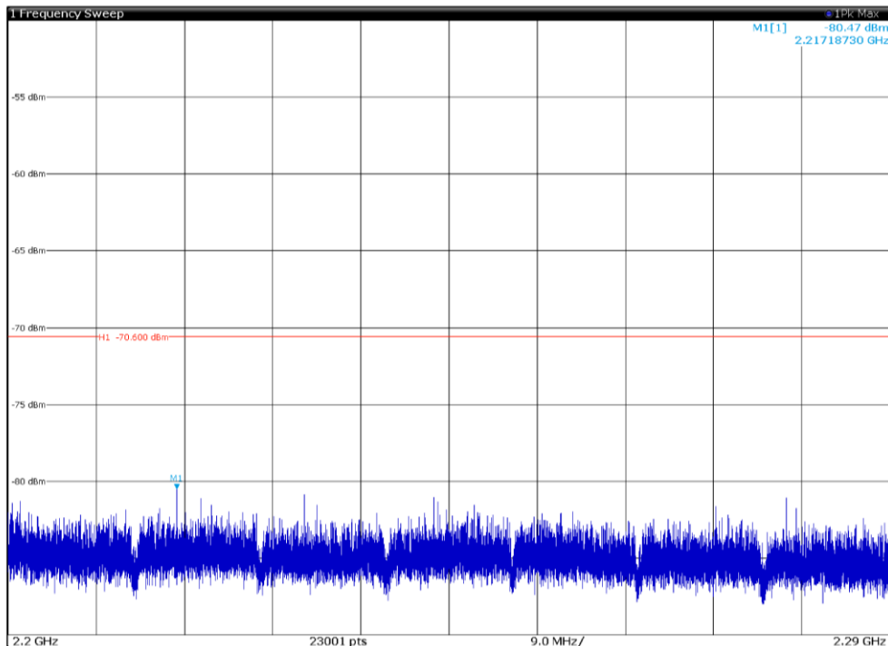
Channel: TOP, Modulation: QPSK, BW=10MHz, Range: 2200MHz-2290GHz, Polarization: Vertical
