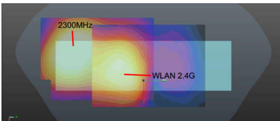
<Flip Opened>: WWAN+WLAN2.4GHz Back 10mm
