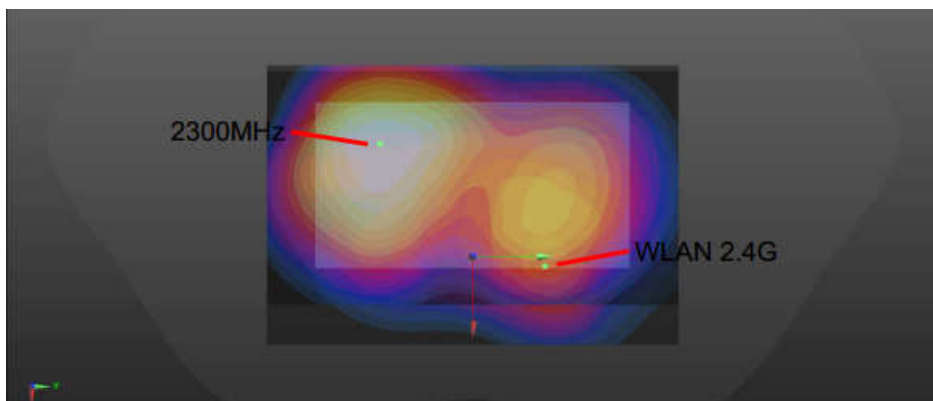
<Flip Closed>: WWAN+WLAN2.4GHz Back 10mm
