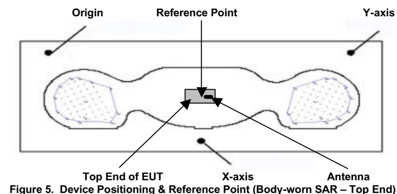
Figure 5. Device Positioning & Reference Point (Body-worn SAR - Top End)
