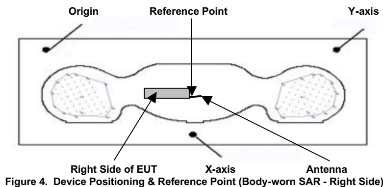
Figure 4. Device Positioning & Reference Point (Body-worn SAR - Right Side)
