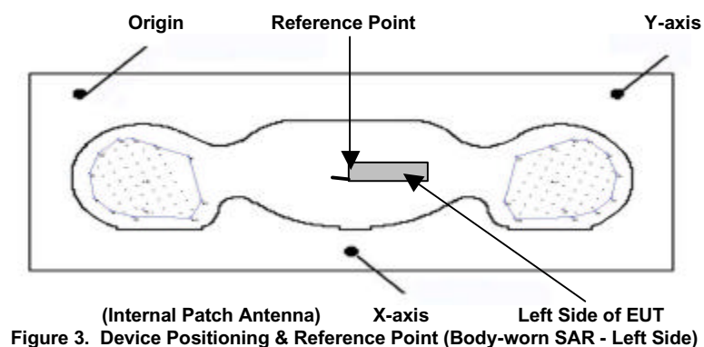
Figure 3. Device Positioning & Reference Point (Body-worn SAR - Left Side)
