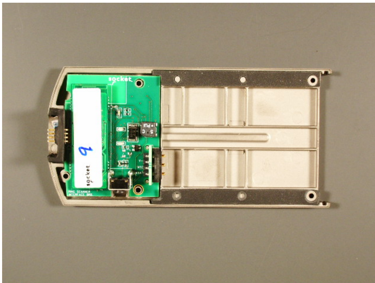
Top Cover Removed
