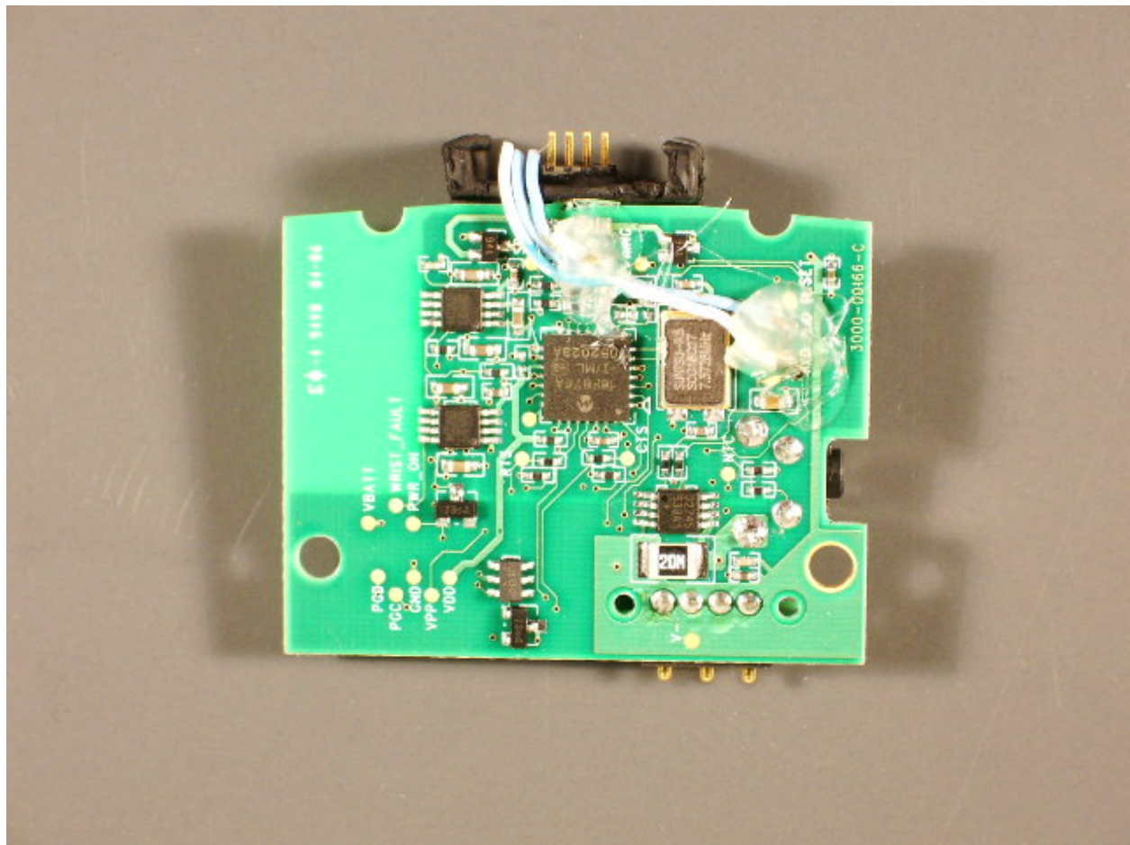
Main PCB – Bottom View
