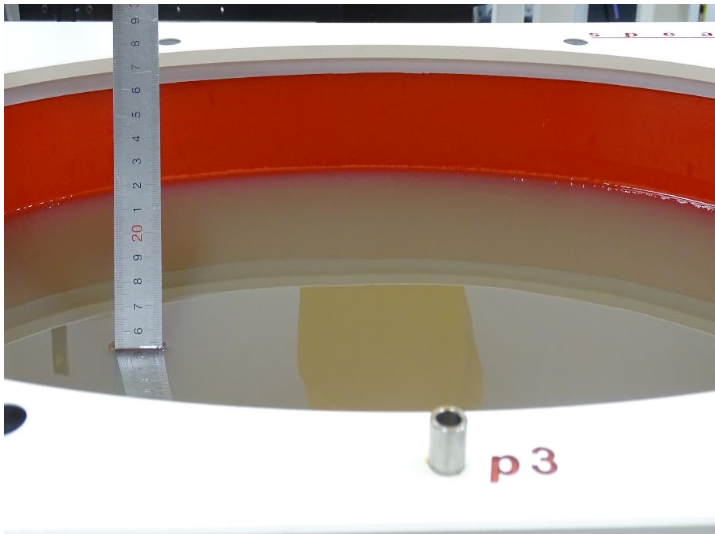
Photo 6: MBBL600-6000MHz Depth (15.1cm)
