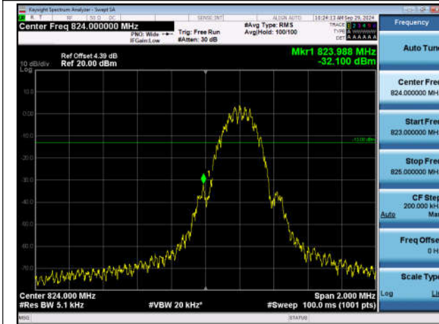
EGPRS850-128-8-PASS
