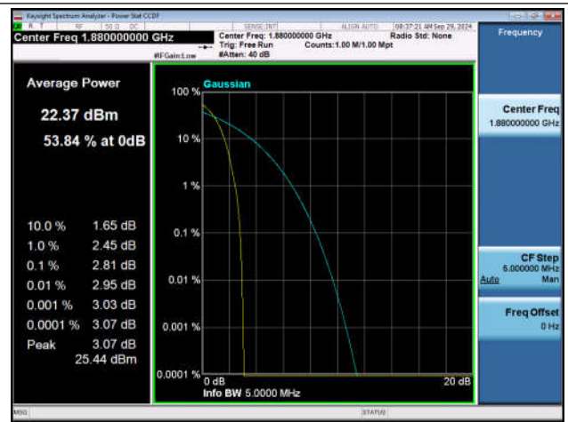
Band2-9400-PASS
