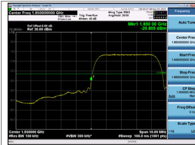
Band2-9262-PASS
