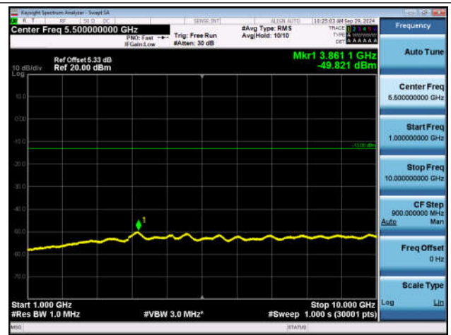
EGPRS850-128-8-1000~10000MHz-PASS
