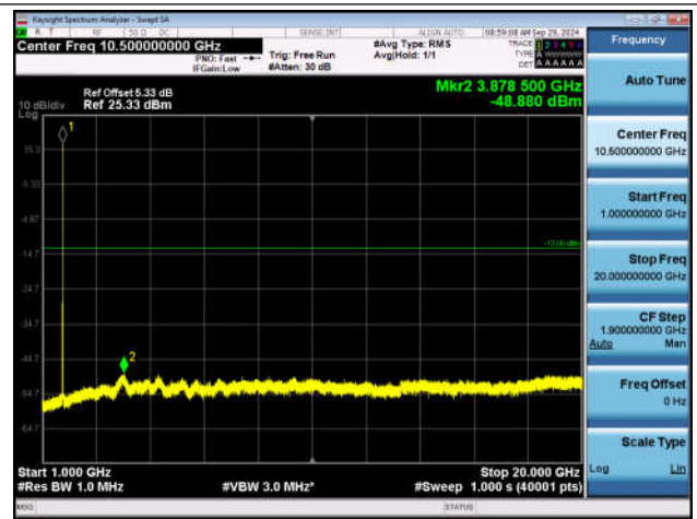
Band4-1312-1000~20000MHz-PASS
