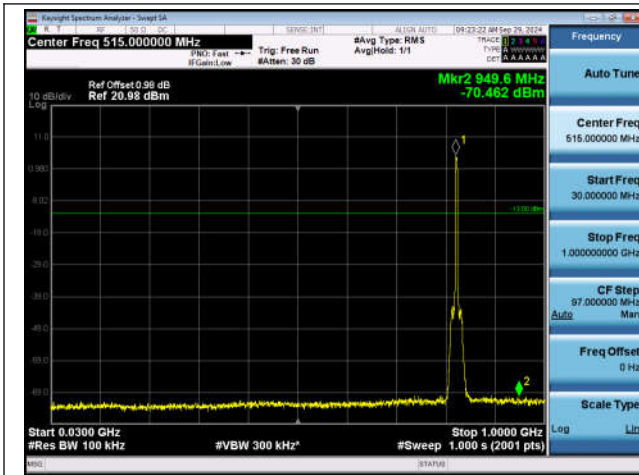
Band5-4132-30~1000MHz-PASS
