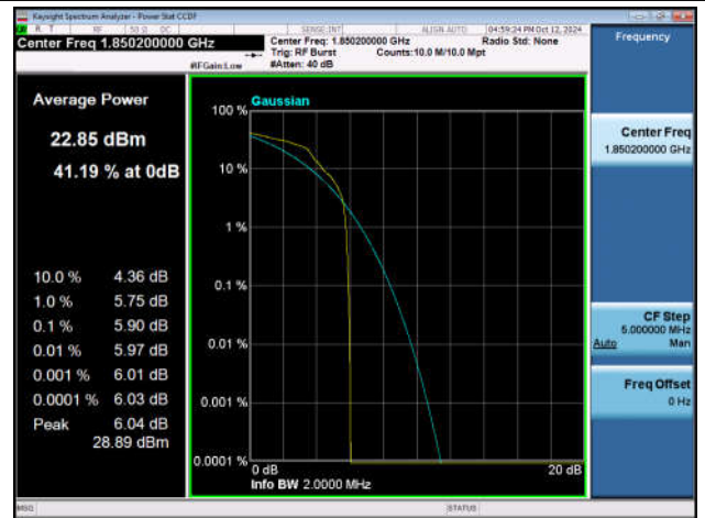
EGPRS1900-512-2-PASS
