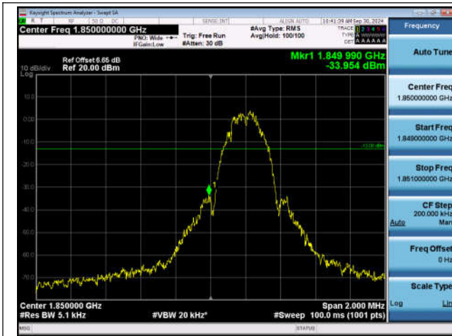
EGPRS1900-512-2-PASS
