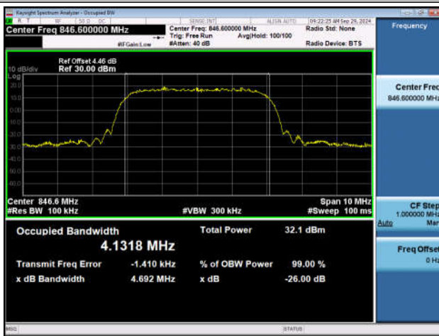
Band5-4233-PASS
