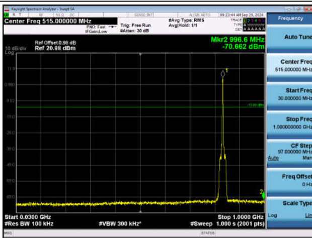
Band5-4183-30~1000MHz-PASS
