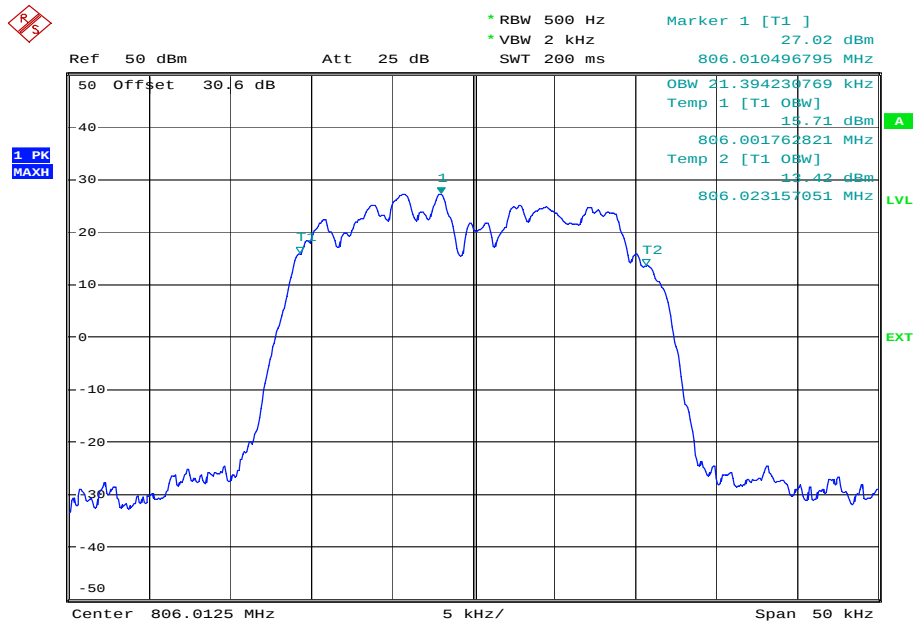
Figure 4 - 806.0125 MHz, Occupied Bandwidth
