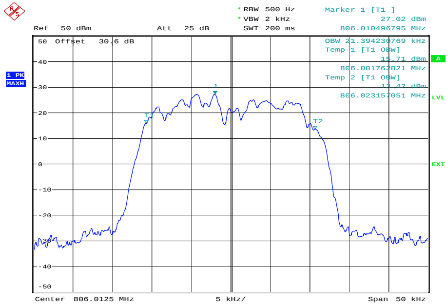
Figure 1 - Frequency Spectrum
