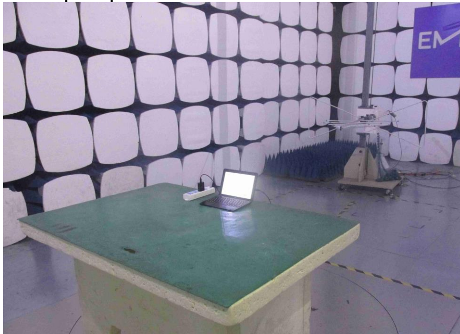
Photograph 2: Set-up for Spurious Emissions for 1 - 18GHz
