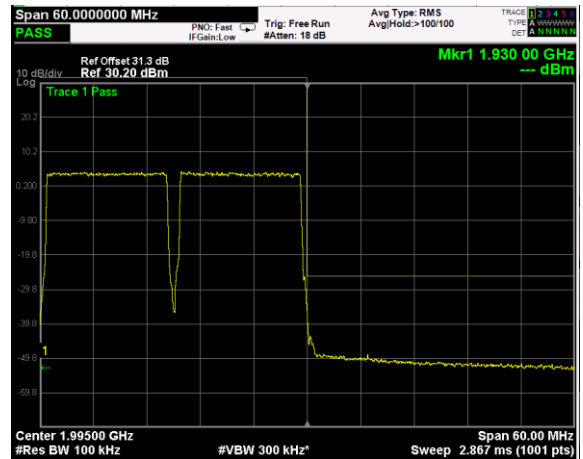
High Band Edge, 2 Carrier, Modulation: QPSK, BW=15MHz
