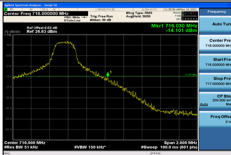
Band17-5MHz-QPSK-23825-1RB#24
