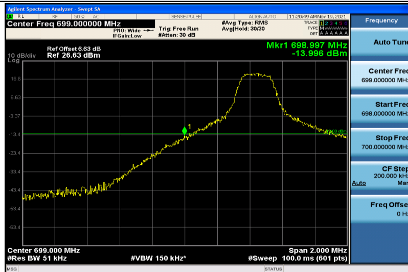
Band12-5MHz-QPSK-23035-1RB#0
