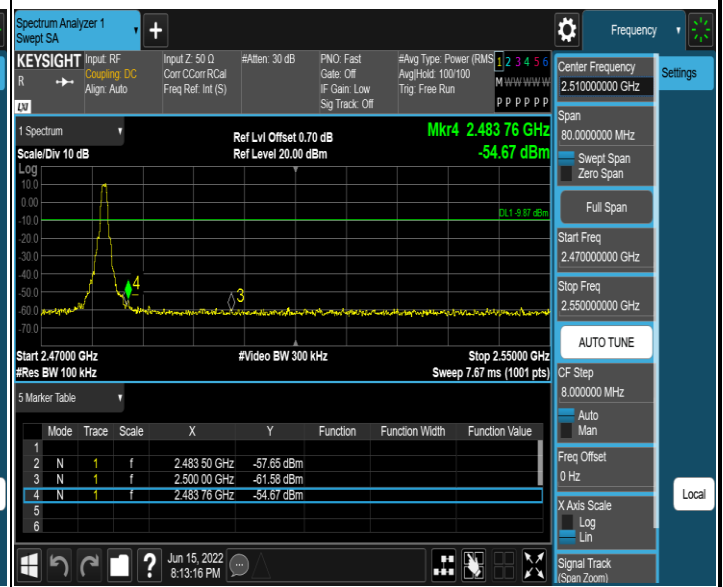
Mode 2 CH39(2480MHz)
