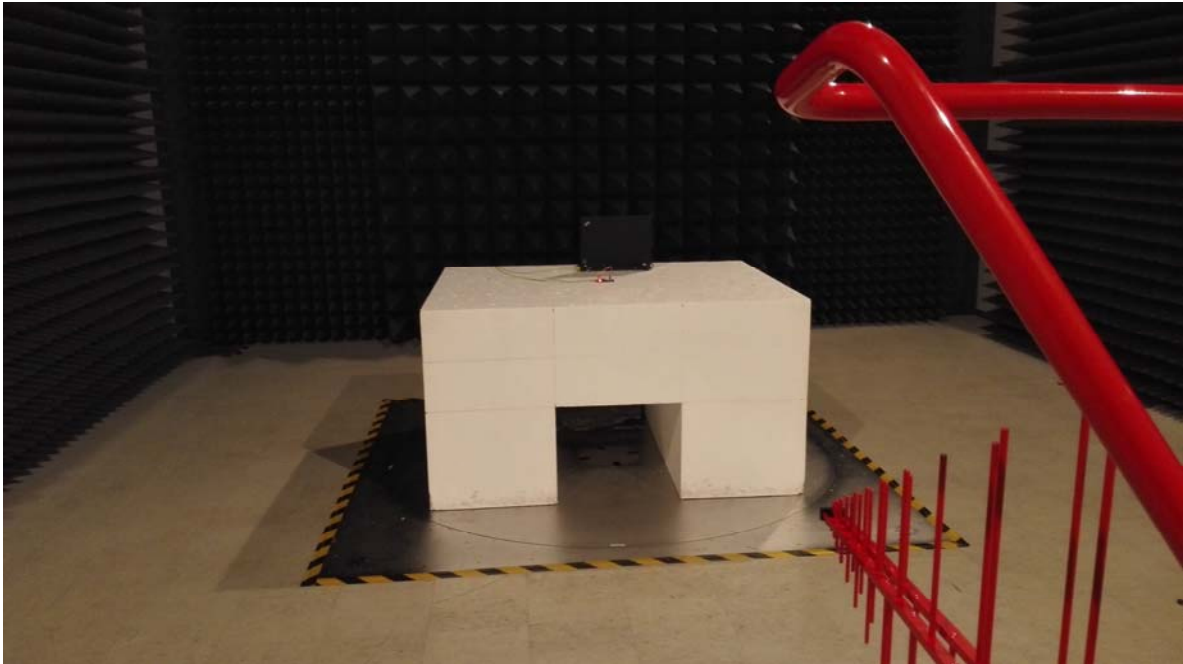
Radiated Spurious Emissions View (Below 1 GHz)
