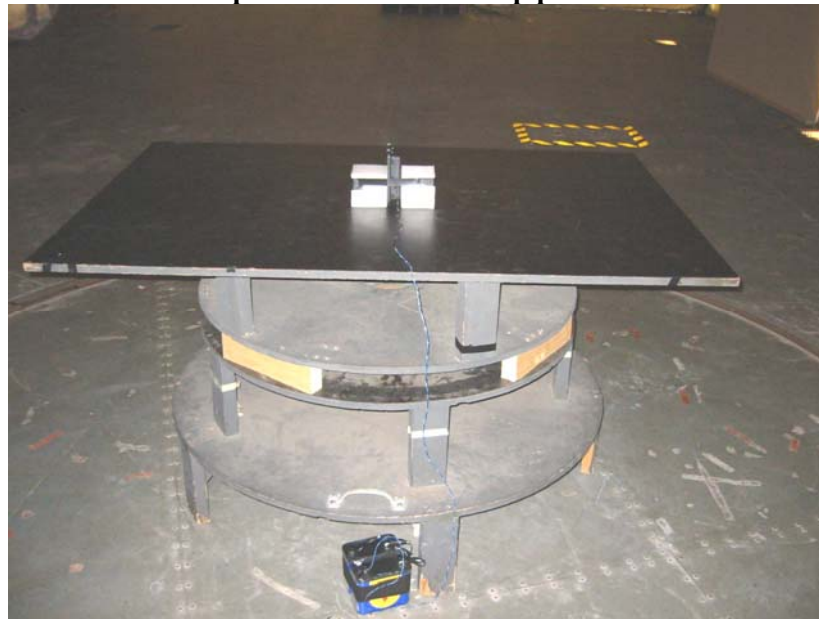
Spurious emissions setup photos
